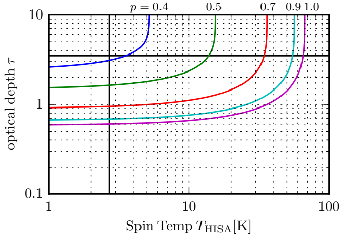
Fig. 4. Optical depth as a function of the spin temperature (as introduced in Eq. (4)) for the region close to the strong continuum source G34.256+0.146 with T_{\text{off}} = 103 K, T_{\text{on}} = 50 K, and T_{\text{cont}} = 17 K. The optical depth of \tau = 3.5 is indicated with a black horizontal line. The temperature of the CMB is indicated at T = 2.7 K with a black vertical line.
