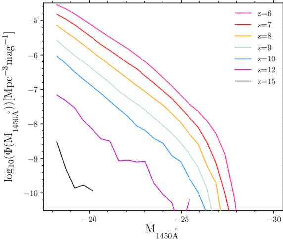
Figure 6. The rest-frame 1450 Å AGN luminosity function predicted by the model at different redshifts, as indicated by the legend.
