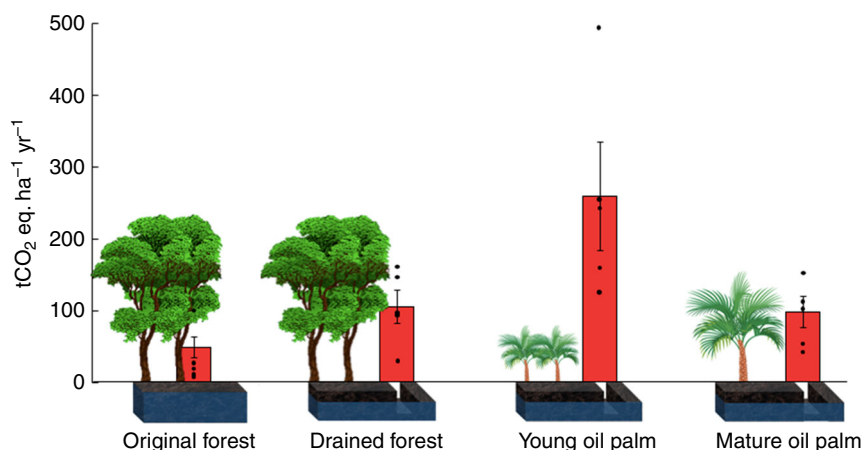
Fig. 3 Emissions factors for each of the four land conversion stages expressed as \text{tCO}_2 \text{eq ha}^{-1} \text{yr}^{-1} accounting for emissions of \text{CO}_2 , \text{CH}_4 and \text{N}_2\text{O} (i.e., accounting for the Global Warming Potential of each of these three gases). Mean and \pm\text{SEM} are shown, \text{SED} = 62.99 , n = 5 . Source data are provided as a Source Data file.
