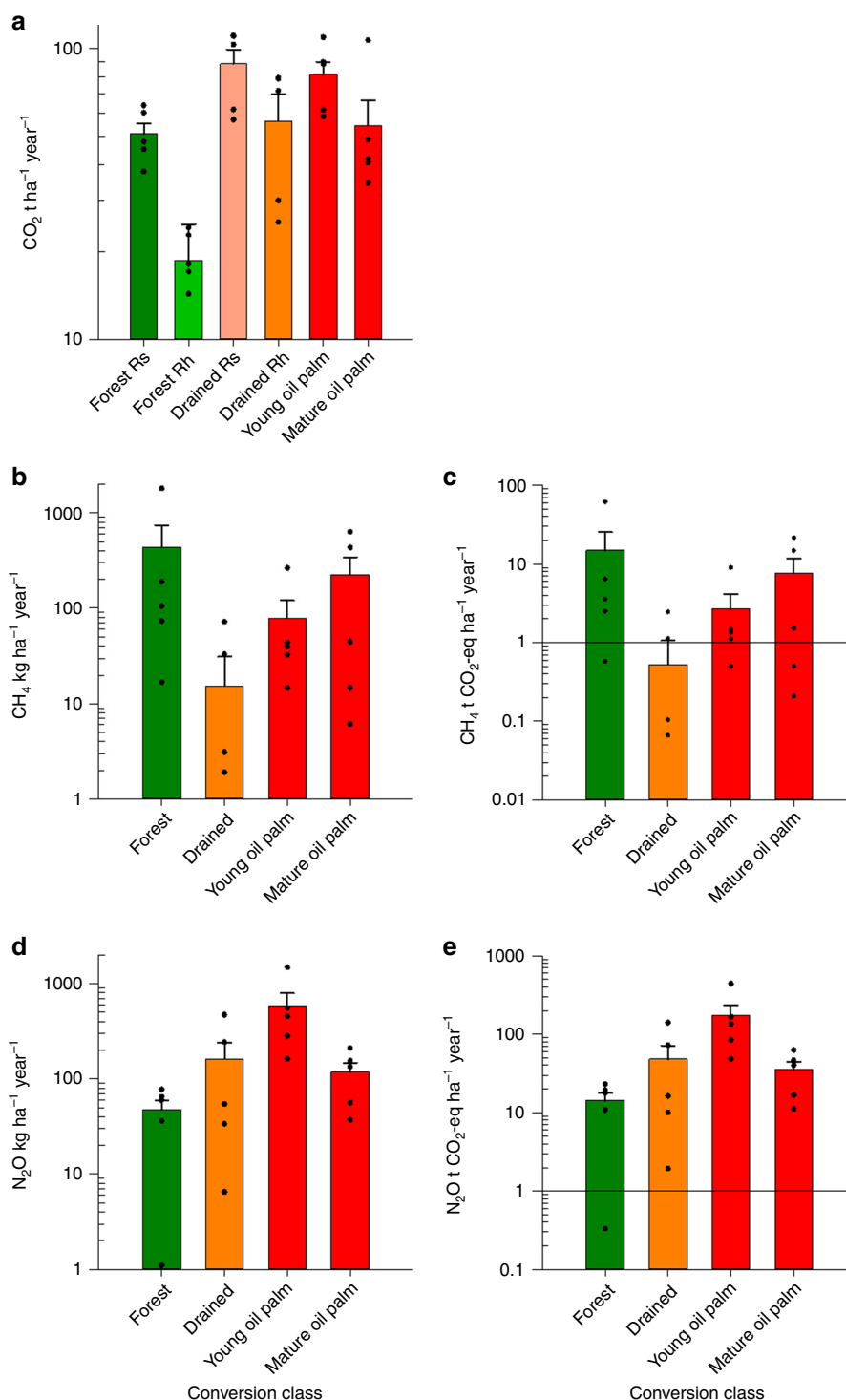
Fig. 2 Greenhouse gas emissions across different land conversion stages. a CO 2 , b and c CH 4 , and d and e N 2 O fluxes from the four class conversion stages expressed as mass fluxes of each individual gas and as CO 2 equivalents (i.e., after accounting for the global warming potential of each of the three gases). At forest and drained sites both heterotrophic respiration (Rh) and overall soil respiration (Rs); at the oil palm sites only Rh was measured. Mean and SEM are shown, n = 5 . Note that a negative CH 4 flux data point at the drained class is not shown as a dot point in panel b and c due to the log scale. Source data are provided as a Source Data file.
