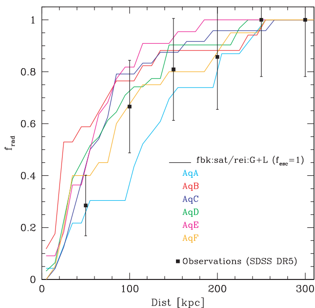
Figure 8. Radial distribution of satellites in the fiducial fbk:sat/rei:G+L model. The observations include both the 11 classical satellites and those detected in the SDSS DR5 (compiled from Mateo 1998 and Koposov et al. 2009), for which the SDSS DR5 threshold selection and sky coverage has been assumed (see text for details). The error bars illustrate the uncertainty due to Poisson statistics. Note that in this cumulative plot, the errors are not independent.
