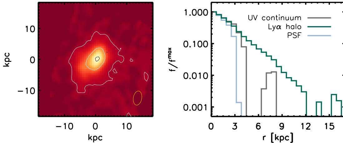
Figure 3. Left: the source-plane reconstruction of the Ly \alpha halo of the lensed galaxy image 4. White contours indicate 50 per cent and 10 per cent of the peak flux in the Ly \alpha halo, while the yellow ellipse in the corner indicates the 50 per cent peak flux for the de-lensed PSF of the MUSE continuum image. The black contour indicates 50 per cent of the peak flux of the UV continuum observed in the HST I_{814} band. The Ly \alpha flux is dominated by a smooth and largely circularly symmetric halo that is extended beyond the stellar continuum, but we also identify an extended region to the south-east (north-west in the image plane). Right: the exponential surface-brightness profile of the Ly \alpha halo, compared to the MUSE continuum (using a foreground-subtracted broad-band image at 7400 Å) surface-brightness profile and the MUSE PSF measured from the source-plane reconstruction of galaxy image 4. The Ly \alpha halo is extended beyond the stellar component measured from the UV continuum.
