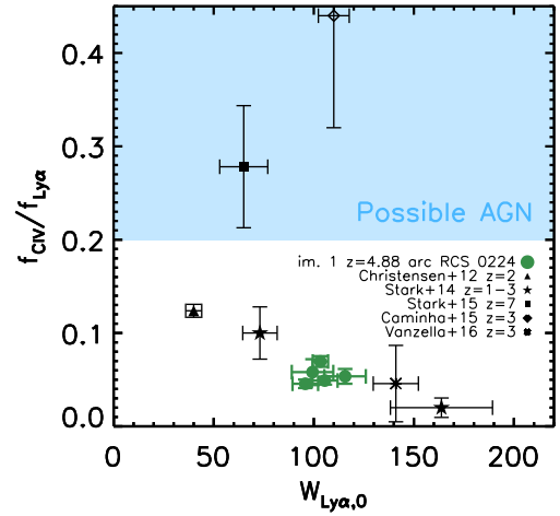
Figure 6. Comparison of the emission-line ratio C IV/Ly \alpha as a function of rest-frame Ly \alpha EW with similar detections in the literature. We show the measurements along the lensed image 1 of the z = 4.88 arc. We also show data from lensed C IV emitters at z \sim 2 found by Christensen et al. (2012b), Stark et al. (2014), Stark et al. (2015), Caminha et al. (2016) and Vanzella et al. (2016). Narrow-line AGN has been observed to show an emission-line ratio of C IV/Ly \alpha \gtrsim 0.2 (Shapley et al. 2003; Erb et al. 2010; Hainline et al. 2011). Along the z = 4.88 arc, this emission-line ratio is steady and always below C IV/Ly \alpha < 0.1 (see Section 3.2.3).
