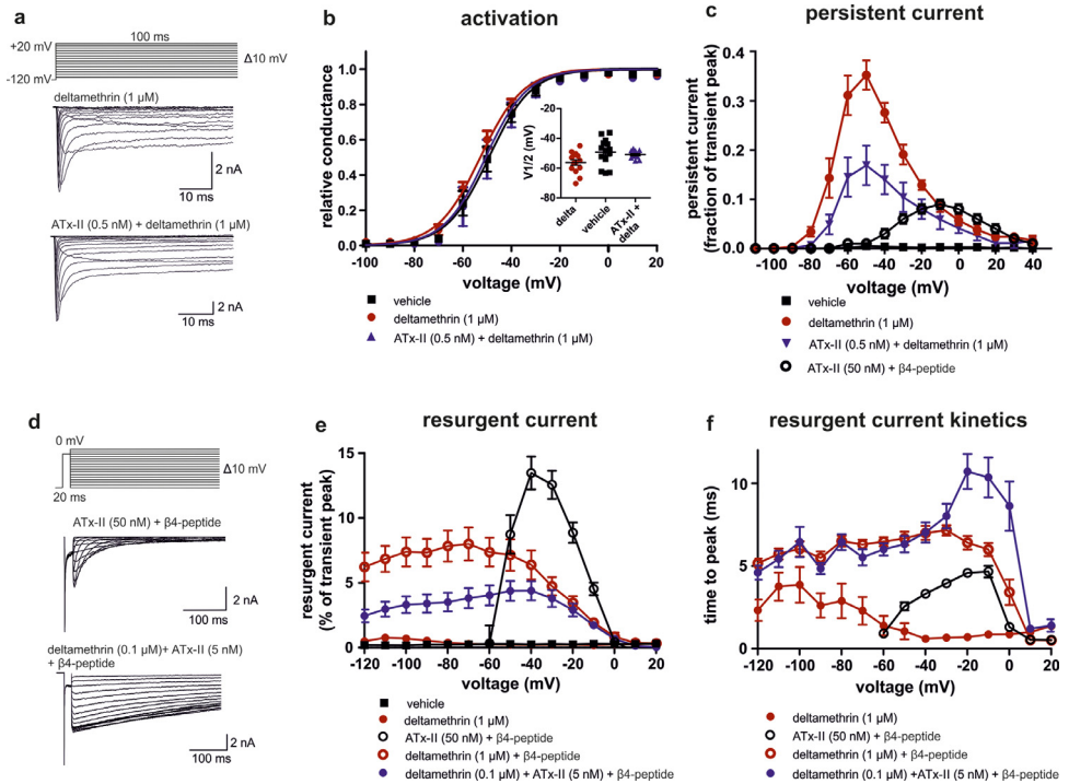
Fig. 3. Effect of ATx-II, deltamethrin and β4-peptide on the gating properties of Nav1.5 channels. (a) Representative voltage protocol and current traces of activating sodium currents during 1 μM deltamethrin and 0.5 nM ATx-II + 1 μM deltamethrin recordings of Nav1.5 in HEK293 cells. (b) Conductance-voltage relationship of Nav1.5 in vehicle, 1 μM deltamethrin or 0.5 nM ATx-II + 1 μM deltamethrin recordings. Conductance was analyzed with leak and zero offset subtraction and normalized to the maximum conductance of each individual cell. Values for half maximal voltage-dependent activation ( V_{1/2} ) were obtained from Boltzmann fits: vehicle -49.2 \text{ mV} \pm 2.4 \text{ mV} (black, n = 14 ); 1 μM deltamethrin -56.2 \text{ mV} \pm 1.9 \text{ mV} (red, n = 14 , p = 0.03 , difference between means = -7.0 \text{ mV} \pm 2.6 \text{ mV} , 95% CI -13.6 \text{ mV} to -0.5 \text{ mV} , t -ratio = 2.7 vs. Vehicle; p = 0.2 , difference between means = -5.3 \text{ mV} \pm 2.7 \text{ mV} , 95% CI -12.1 \text{ mV} to 1.5 \text{ mV} , t -ratio = 2.0 vs. 0.5 nM ATx-II + 1 μM deltamethrin); 0.5 nM ATx-II + 1 μM deltamethrin -50.9 \text{ mV} \pm 0.8 \text{ mV} (blue, n = 12 , p > 0.99 , difference between means = 3.4 \text{ mV} \pm 2.7 \text{ mV} , 95% CI -5.1 \text{ mV} to 8.5 \text{ mV} , t -ratio = 0.6 vs. vehicle, one-way ANOVA with a Bonferroni's post-hoc analysis). Conductance of ATx-II + deltamethrin recordings shows no difference to vehicle recordings. (c) Mean persistent current was obtained during the final 13 ms of 100 ms depolarizing pulses in vehicle, 1 μM deltamethrin, 0.5 nM ATx-II + 1 μM deltamethrin and 50 nM ATx-II + 100 μM β4-peptide. Currents were analyzed with leak and zero offset subtraction and normalized to the maximum inward current. Maximum persistent currents at -50 \text{ mV} , evoked by vehicle 0.01 \pm 0.00 (black, n = 19 ), 1 μM deltamethrin 0.35 \pm 0.03 (red, n = 24 ) or 0.5 nM ATx-II + 1 μM deltamethrin 0.17 \pm 0.04 (blue, n = 12 ), and at 0 \text{ mV} , evoked by 50 nM ATx-II + 100 μM β4-peptide 0.08 \pm 0.01 (unfilled black, n = 14 ). The combination of ATx-II and deltamethrin and ATx-II and β4-peptide generates smaller persistent currents than deltamethrin alone. Also note the different voltage dependence of ATx-II + β4-peptide persistent currents. (d) Representative resurgent current traces evoked by the indicated voltage protocol recorded in 50 nM ATx-II + 100 μM β4-peptide and 0.1 μM deltamethrin + 5 nM ATx-II + 100 μM β4-peptide recordings in Nav1.5 channels. (e) Resurgent currents were determined and analyzed as in Fig. 2a (gray box) and normalized to the maximum inward current of the depolarizing pre-pulse. Resurgent currents evoked by vehicle (black, n = 16 ); 1 μM deltamethrin (filled red, n = 16 ); 50 nM ATx-II + 100 μM β4-peptide (unfilled black, n = 15 ); 1 μM deltamethrin + 100 μM β4-peptide (unfilled red, n = 13 ); and 0.1 μM deltamethrin + 5 nM ATx-II + 100 μM β4-peptide (filled blue, n = 17 ). ATx-II and β4-peptide resurgent currents were depicted from -60 \text{ mV} since the combination does not produce resurgent currents at more negative potentials [1]. Resurgent currents of combinations including β4-peptide are generally larger than deltamethrin-induced resurgent-like currents. Note the different voltage dependence of ATx-II and β4-peptide resurgent currents. Also note the tenfold smaller deltamethrin concentration of the combination of ATx-II + deltamethrin + β4-peptide (filled blue circles) compared to previous measurements. (f) Time-to-peak of the resurgent current was measured in individual recordings and plotted against the repolarization voltage: 1 μM deltamethrin (filled red, n = 20 ), 50 nM ATx-II + 100 μM β4-peptide (unfilled black, n = 15 ), 1 μM deltamethrin + 100 μM β4-peptide (unfilled red, n = 17 ), ATx-II and β4-peptide (unfilled blue, n = 19 ). Resurgent-like currents induced by either deltamethrin or β4-peptide alone are generally faster than those induced by combinations including deltamethrin and β4-peptide. (For interpretation of the references to color in this figure legend, the reader is referred to the web version of this article.)
