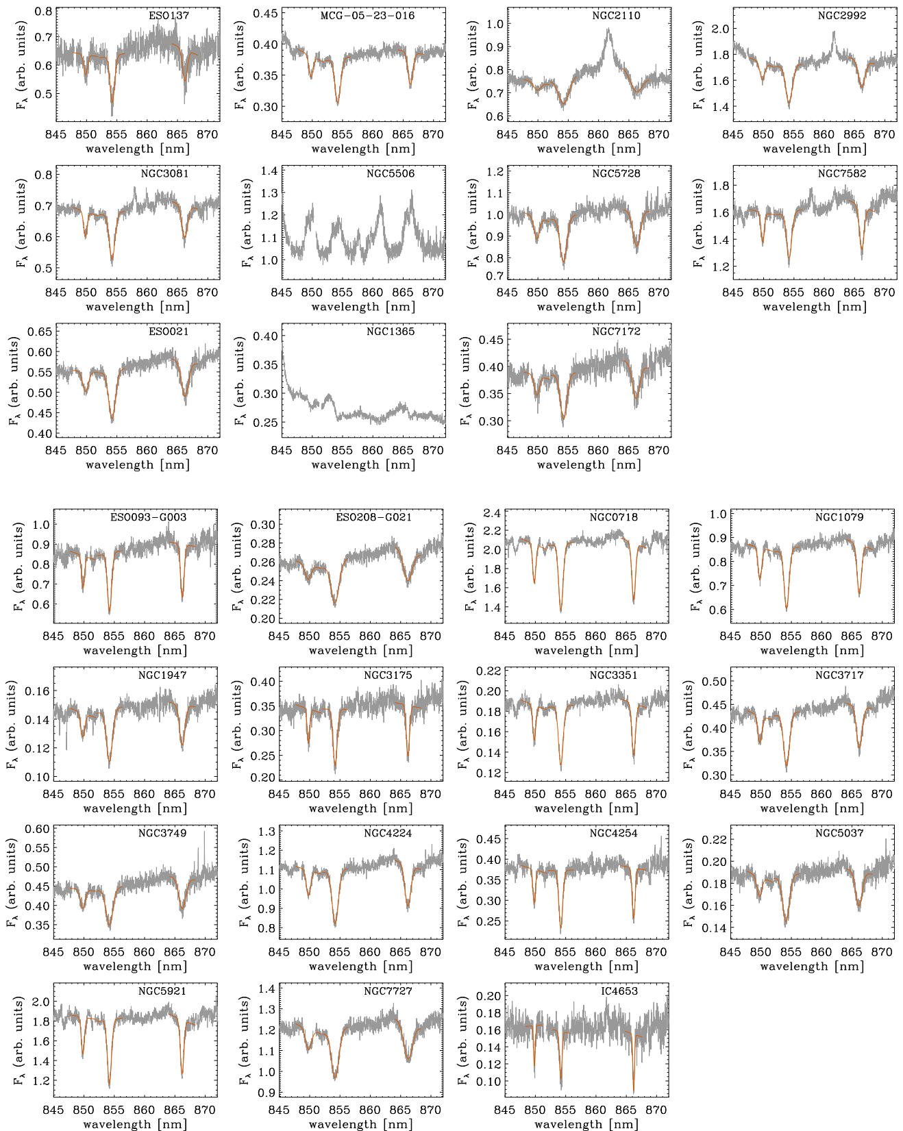
Figure A1. Fits to the Ca II triplet lines for one spectrum of each active galaxy (upper 11 panels) and inactive galaxy (lower 15 panels). Only the data are shown for NGC 1365 and NGC 5506 because there were no clear absorption lines to fit. The data are shown in grey and the fits in red. A Gaussian line profile was fitted independently to each line in order to avoid bias due to the continuum shape and emission lines. The arbitrary units of F_\lambda are the same for all panels.
