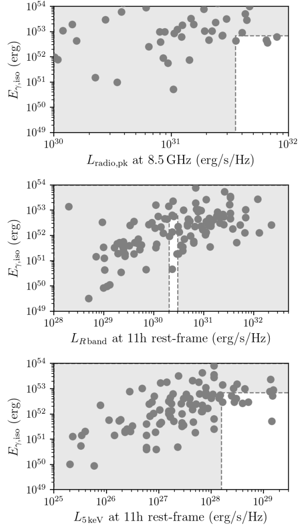
Figure 3. Optical, X-ray, and radio afterglow luminosity of classical GRB afterglows in the literature, compared to the isotropic gamma-ray energy release E_{\gamma, \text{iso}} (grey circles). The optical and X-ray afterglow values were taken from Figure 5 and Figure 6 of Nysewander et al. (2009), and the radio afterglow values were taken from Figure 20 of Chandra & Frail (2012). The region shaded in grey indicates the phase-space ruled out for AT 2020blt based on our observations and an upper limit on E_{\gamma, \text{iso}} from KONUS-Wind . We cannot rule out the possibility that AT 2020blt was a classical GRB afterglow missed by high-energy detectors.
