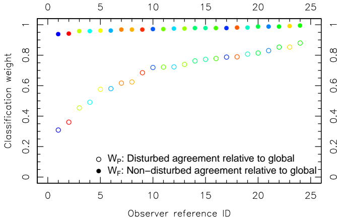
Figure A2. Comparison of classification weights for individual classifiers (24 in total). The classifiers are ordered by their W_F weight, i.e. how consistently their ‘undisturbed’ classification agrees with that of their fellow classifiers. The y-axis indicates the weight used to re-define classification assessments. If a classifier tends to generously flag galaxies as disturbed compared to the global typical classification (left hand side) their weight for such an assessment is decreased. This is not to say the global choice is always better , but for this analysis we want all classifications to be biased in the same way.
