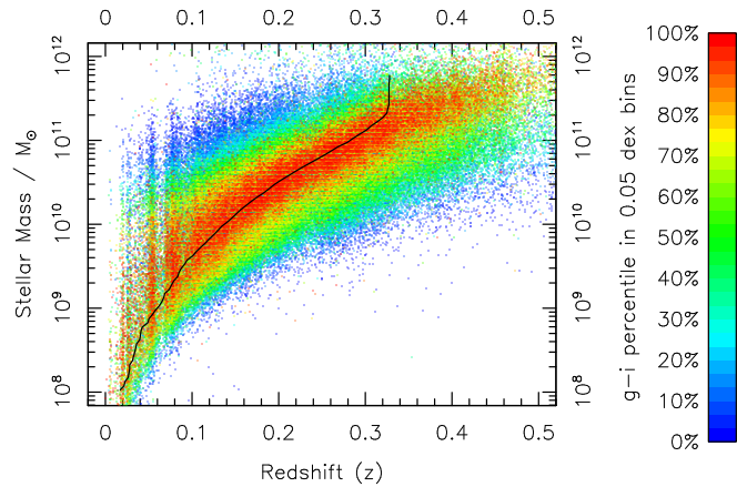
Figure 1. The variable stellar mass redshift selection limit. In each vertical M \pm 0.025 dex bin the cumulative density function (CDF) of apparent g-i colour is calculated. Depending on where a galaxy appears in the CDF given its stellar mass the colour of the data point is different: relatively bluer (redder) g-i colour galaxies are bluer (redder) data points. The black line shows the selection limit and is imposed at the 95 th percentile for each bin.
