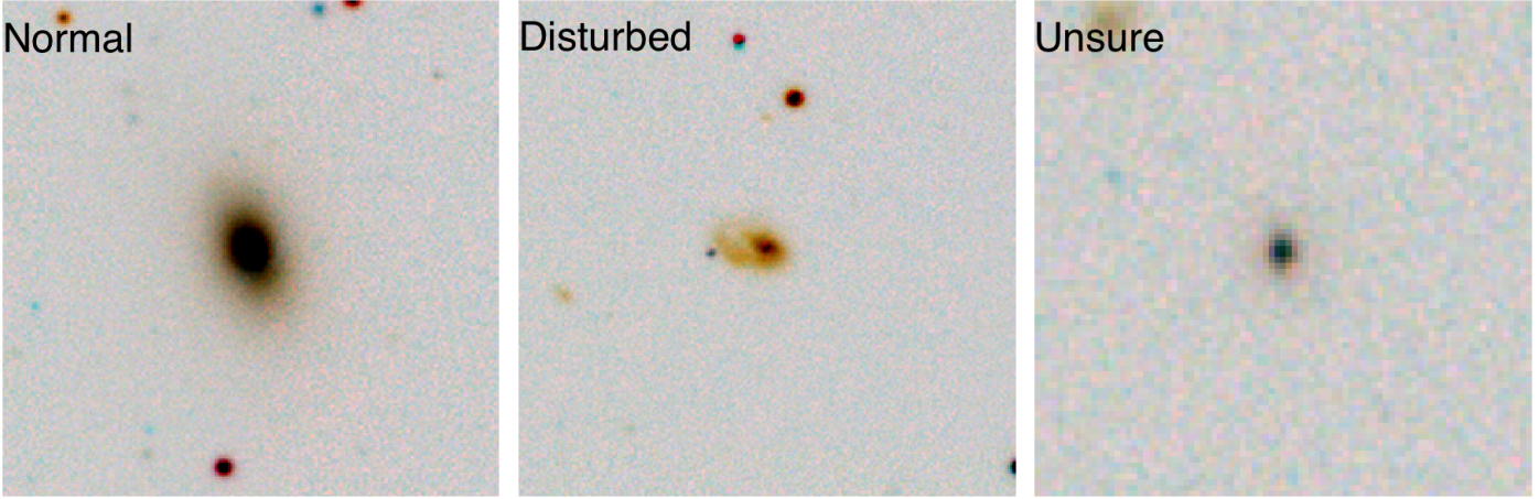
Figure A1. The three classifications of galaxy disturbance used in this work. All images used are 60 h^{-1} \text{ kpc} \times 60 h^{-1} \text{ kpc} in physical distance and linearly map g/r/K SDSS and VIKING flux data onto blue, green and red colours which are then inverted. This means visually redder colours correspond to bluer g-r colours in the original images. The left panel is an example of a ‘normal’ galaxy that does not show signs of morphological disturbance, the middle panel is an example of a ‘disturbed’ galaxy and the right panel is an example of a galaxy where our classification would be ‘unsure’ because there are so few pixels of information. Images were randomly selected from the close-pairs subset (i.e. all of them have known close-pair companion galaxies, and none are taken from the isolated control sample).
