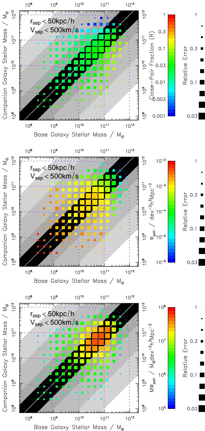
Figure 8. Pair properties for r_{\text{sep}} < 50 \text{ kpc} and v_{\text{sep}} < 500 \text{ km s}^{-1} sample ( PS_{r20v500} ) true pair corrected using the mock catalogues ( W_{TP\text{-}mock} , see Section 3.4). For more information see the caption for Figure 7.
