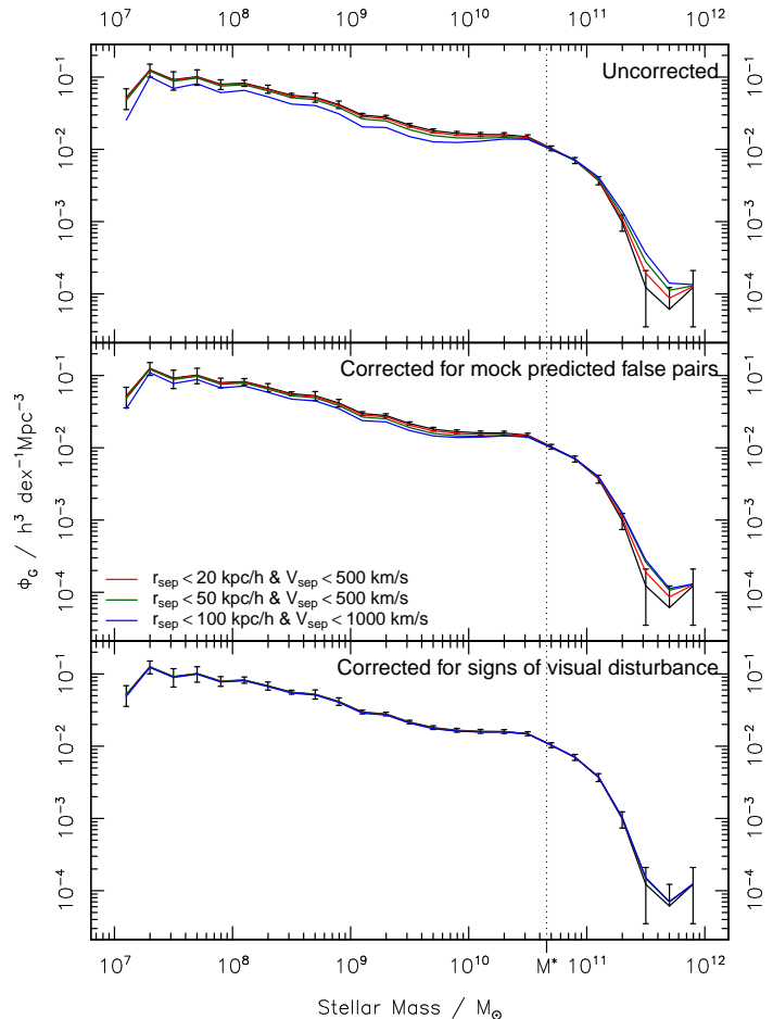
Figure 18. Depiction of the effect on the GSMF presented in Baldry et al. (2012) if the different close-pair selections shown in Figure 16 were assumed to merge on some unknown timescale. The top panel is only corrected for galaxies appearing in multiple close-pairs. The middle panel is true pair corrected from the mock catalogues using W_{TP-mock} (see Section 3.4). The bottom panel is corrected for the fraction of visually disturbed galaxies in pairs using W_{TP-vc} (see Section 3.4). In all cases mass is moved from moderate stellar mass galaxies ( 10^8 M_\odot – 10^{10} M_\odot ) to beyond \mathcal{M}^* (although this is hard to identify in the bottom panel). This has the inevitable effect of enhancing the dip in this regime, increasing the significance of the double-Schechter shape in the GSMF and moving the future value of the GSMF \mathcal{M}^* to larger masses.
