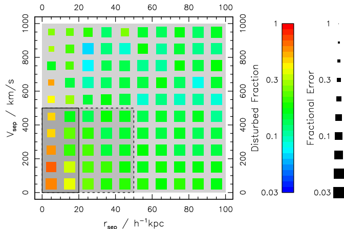
Figure 6. Fraction of galaxies in each dynamical bin showing signs of disturbance. This is corrected for the simplest stellar mass dependent redshift bias (see Figure 4). The darkest grey box with solid lines shows the PS_{r20v500} sample, the next darkest box with dashed lines shows the PS_{r50v500} sample, and the entire plotting region shows the PS_{r100v1000} sample. The size of the box indicates the error, where smaller means less significant, i.e. more error in the measurement.
