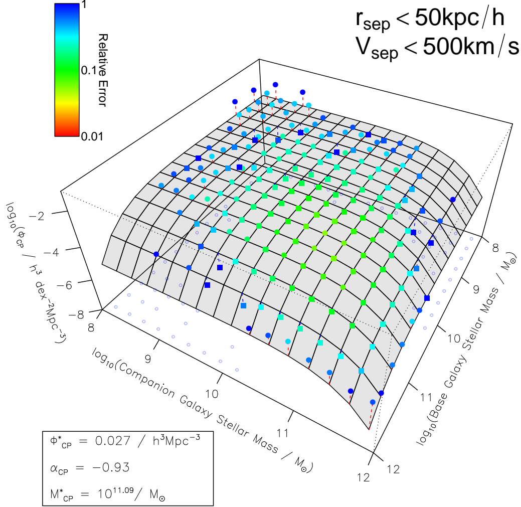
Figure 11. Fit to the 2D close-pair density distribution for r_{\text{sep}} < 50 \text{ kpc} and v_{\text{sep}} < 500 \text{ km s}^{-1} sample ( PS_{r20v500} ) as observed, i.e. not true pair corrected using the mock catalogues (see Section 3.4). See Figure 10 for details.
