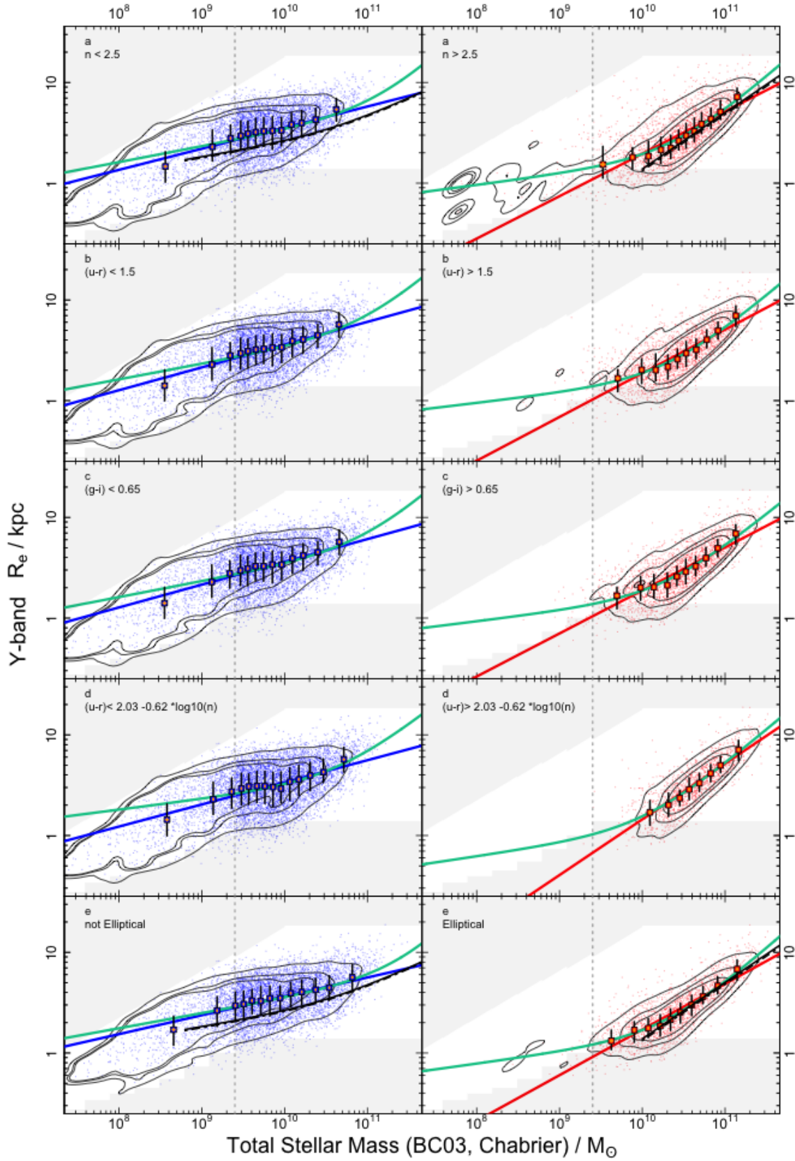
Figure A6. The M_* - R_e relation for the Y-band with the panels and fits as in Fig. A1.
