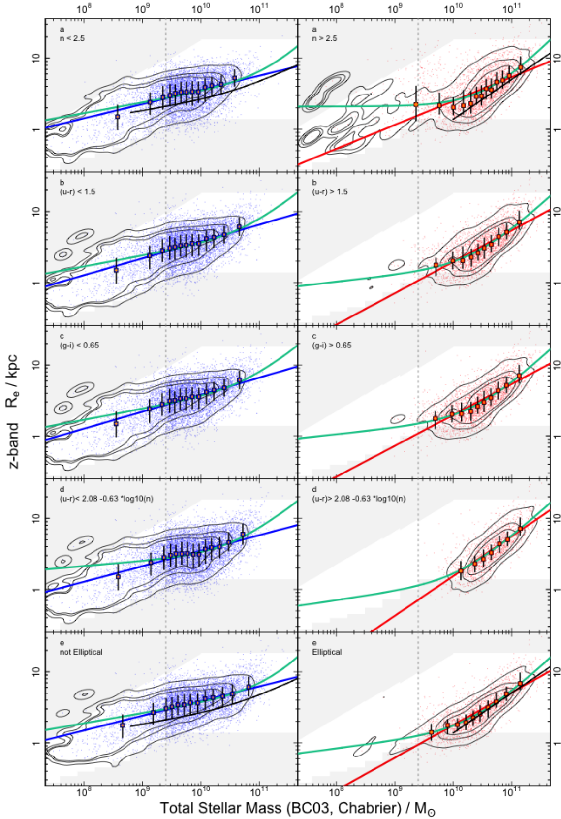
Figure A4. The M_* - R_e relation for the z-band with the panels and fits as in Fig. A1.
