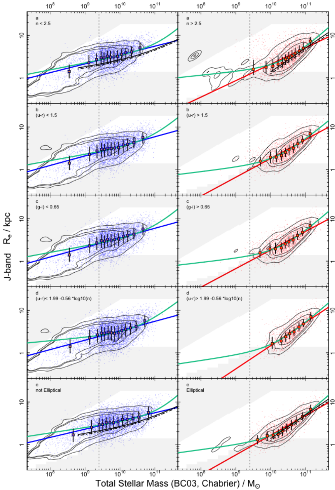
Figure A7. The M_* - R_e relation for the J-band with the panels and fits as in Fig. A1.
