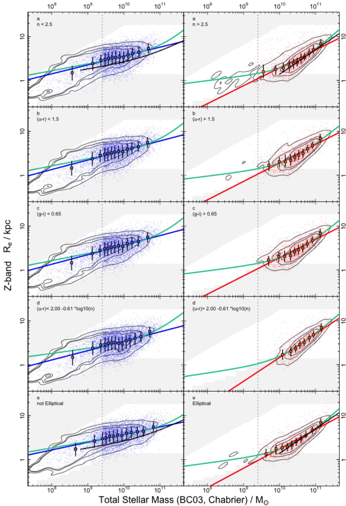
Figure A5. The M_* - R_e relation for the VIKING Z-band with the panels and fits as in Fig. A1.
