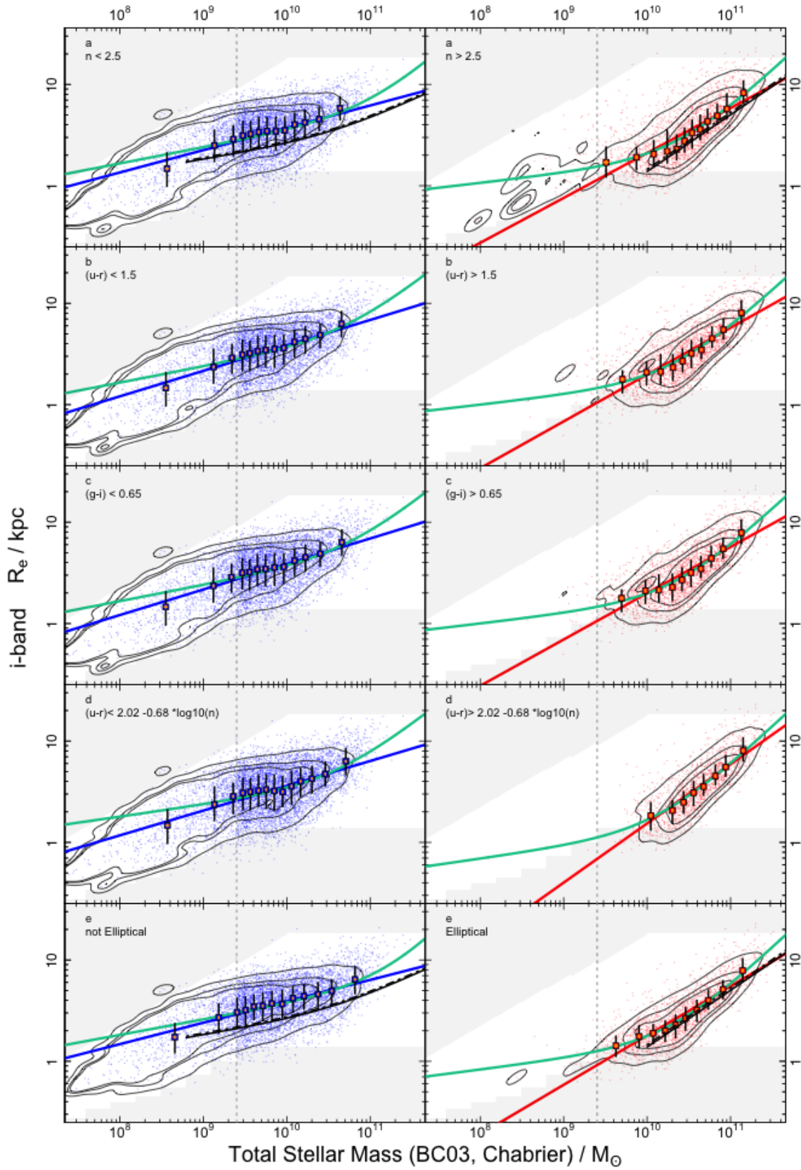
Figure A3. The M_* - R_e relation for the i -band with the panels and fits as in Fig. A1.
