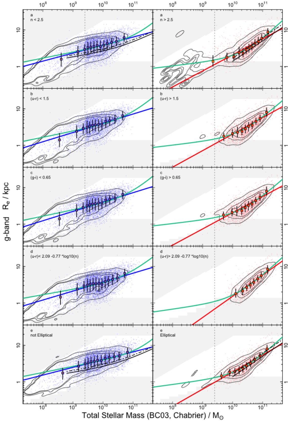
Figure A2. The M_* - R_e relation for the g -band with the panels and fits as in Fig. A1.
