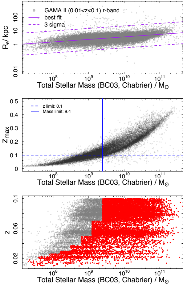
Figure 1. (Top) The stellar mass – (major axis) half-light radius distribution of the sample extracted from the GAMA catalogue with all galaxies in the redshift range 0.01 < z < 0.1 as grey dots, the solid purple line shows an initial least square fit to the entire data set and the dashed lines indicate the 3\sigma scatter. Galaxies more than 3\sigma away from the best fit are excluded from the final data set.
