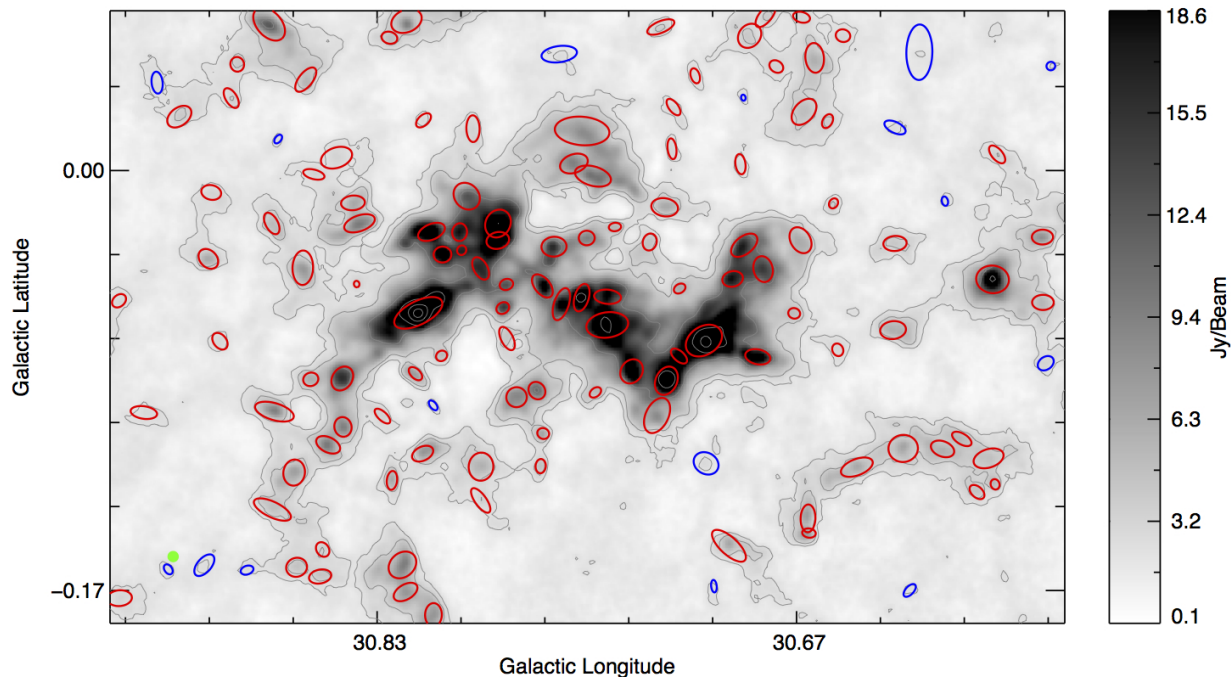
Figure 8. Example of the source-extraction results in a small portion of the \ell = 30^\circ region. The greyscale image shows the 850- \mu\text{m} emission and the red and blue ellipses show the approximate sizes and orientations of the sources above and below 5\sigma . The grey contours start at 3\sigma and increase in steps of 0.17, 0.8, 2.75, 6.81, 13.85 \text{Jy beam}^{-1} . The green filled circle in the lower-left corner indicates the FWHM size of the JCMT beam at 850 \mu\text{m} .
