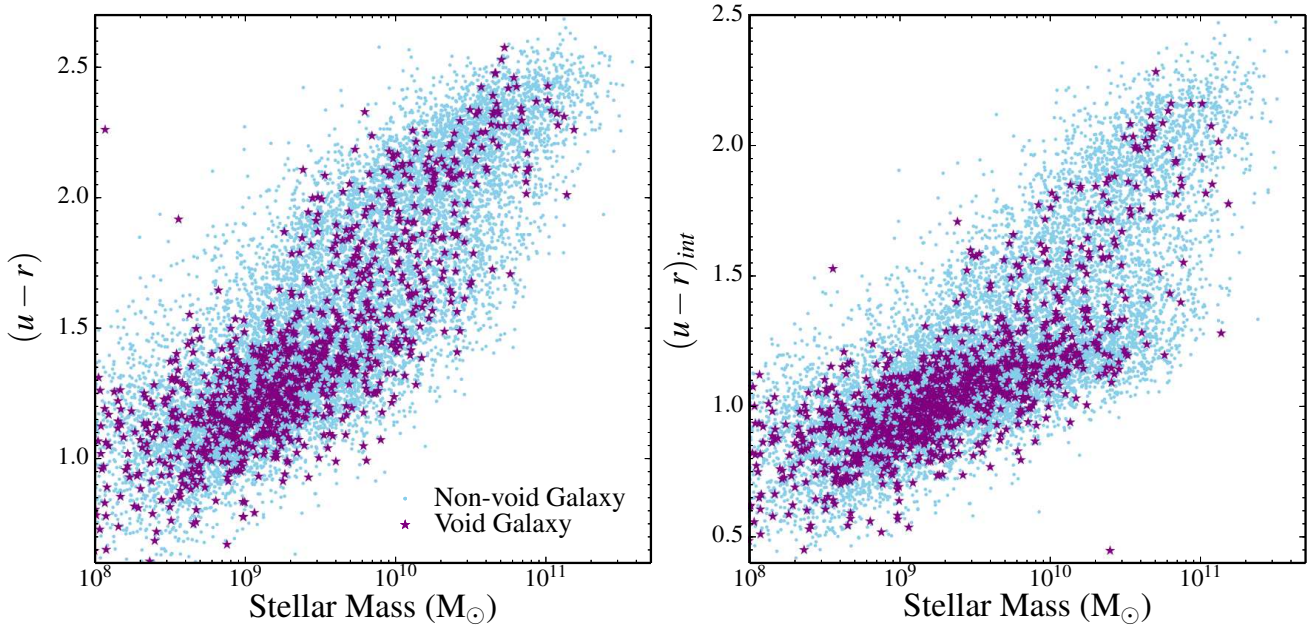
Figure 4. Colour-mass relation for GAMA void galaxies (purple stars). The left-hand panel shows rest-frame (u - r) observed colours, with the rest-frame intrinsic (u - r)_{int} colours (corrected for internal dust reddening) shown in the right-hand panel. The colours have been k -corrected to z = 0 in both plots, and corrected for foreground extinction. Also shown are non-void galaxies for comparison (blue dots). The majority of void galaxies are low mass, blue, star forming irregular and spiral galaxies. A red sequence is seen for both the void and non-void galaxy populations, which remains after the colours have been corrected for internal dust reddening.
