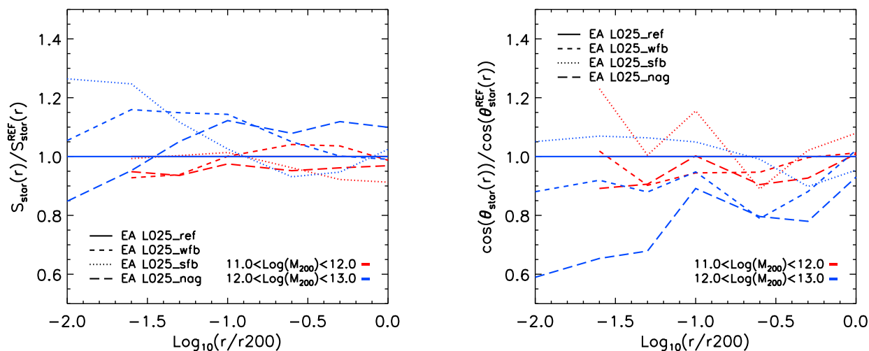
Figure 2. Ratios of the average sphericity (left panel) and average misalignment angles (right panel) of the stellar distribution with respect to the average values of the REFERENCE EAGLE simulation (see §3). Different colours indicate different mass bins while different line styles refer to different simulations which differ only by the implementation of feedback. The disagreement (up to 20% for sphericity and up to 40% for misalignment angle) stems from the different efficiency of galaxy formation (see discussion in §3). The misalignment angle is more sensitive to galaxy formation efficiencies than the sphericity. The differences always increase towards the centre of the halo.
