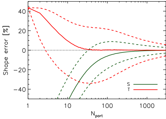
Figure A1. Convergence test for shape parameter retrieval. Relative error on the retrieved shape parameter of a synthetic NFW halo as a function of the number of particles used to sample the underlying distribution. The relative errors on sphericity and triaxiality are indicated by the green and red lines, respectively. The test is performed using a typical sphericity value for the synthetic halo, S = 0.6 and T = 0.7 . For each number of particles, distributions are drawn 10^5 times and we report the 50th (continuous lines), 16th and 84th percentiles (dashed lines). Retrieving both shape parameters with a systematic error smaller than a few percent requires at least 300 particles.
