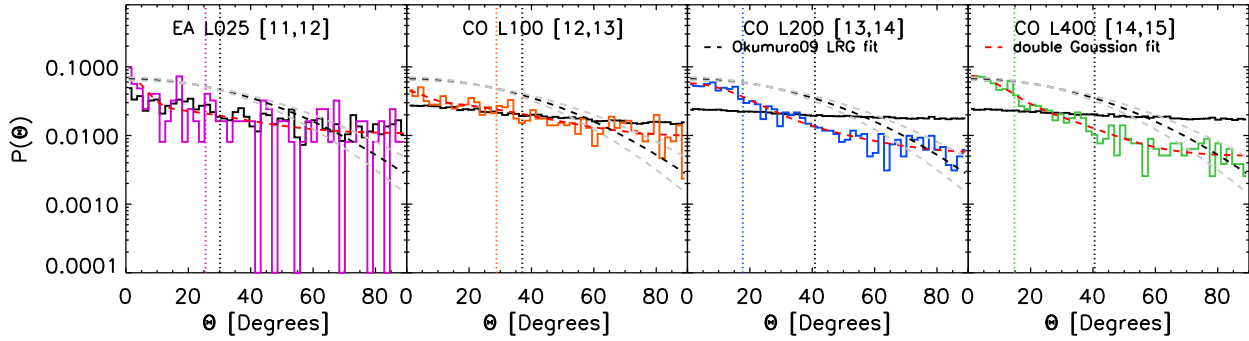
Figure 10. Probability distribution function of the 2D misalignment angle between the major axes of the projected distribution of stars (inside r_{\text{half}}^{\text{star}} ) and the major axes of the projected total matter distribution for four halo mass bins. The black histograms indicate the probability distributions for the total sample of haloes that satisfies the resolution criteria, whereas coloured histograms refer only to the subsample of haloes whose mass is indicated in the legend. Vertical lines indicate the median values of the misalignment angle (same colour convention as for the histograms). Red dashed curves represent the analytic fit discussed in Appendix B, whereas black and grey curves are obtained with analytic functional forms that have been employed in the literature (see text).
