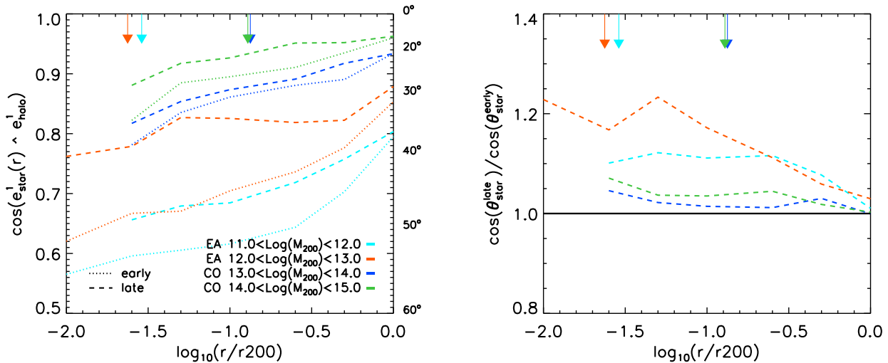
Figure 11. Left Panel. Spatial variation of the cosine of the median misalignment angle between stars and the underlying (mostly dark) matter distribution. Different colours refer to different halo mass bins, whereas different line styles refer to different galaxy types. Radii are rescaled to the mean halo radius, r_{200}^{\text{crit}} , to ease the comparison of the results corresponding to different halo mass bins. Only central haloes are used in order to remove effects that can alter mostly the alignment of satellites. Here the direction of the halo is determined using all particles belonging to the structure. A kinematic classification has been employed (see text) to divide galaxies into early- and late-type. Right Panel. Spatial variation of the ratio between the alignment of late and early type galaxies. As in the left panel, the alignment is expressed in terms of the cosine of the angle between galaxy and halo major axes. In both panels the least massive bin is taken from the L100 simulation to improve on the otherwise poor statistics of L025. The vertical arrows represent the median values of r_{\text{half}}^{\text{star}} in units of r_{\text{crit}}^{200} in different mass bins.
