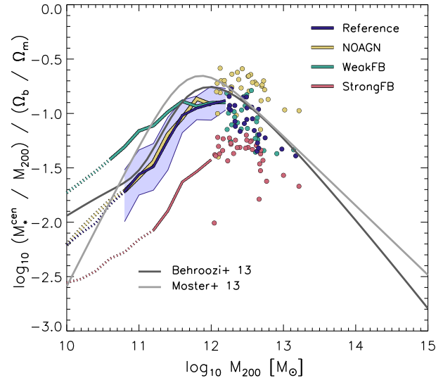
Figure 1. The stellar mass to halo mass ratio of central galaxies as a function of halo mass, normalised by the cosmic baryon fraction, for the four feedback variations used in §3. The curves are dotted where there are fewer than 100 star particles per galaxy and individual galaxies are shown for bins that contain fewer than 10 galaxies. The 1-sigma scatter about the median of Reference is shown as a shaded region. Dark and light grey lines represent the abundance matching relations of Behroozi, Wechsler & Conroy (2013) and Mozer, Naab & White (2013).
