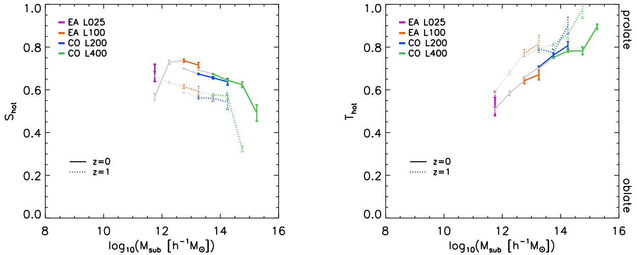
Figure 7. Shape parameters (sphericity on the left, triaxiality on the right) of the gas distribution for the hot ( T > 10^6 \text{K} ) component. Different colours indicate different simulations, whereas different line styles refer to different redshifts. The error bars represent one sigma bootstrap error on the median. Grey lines show the results for mass bins containing haloes with less than 300 hot gas particles.
