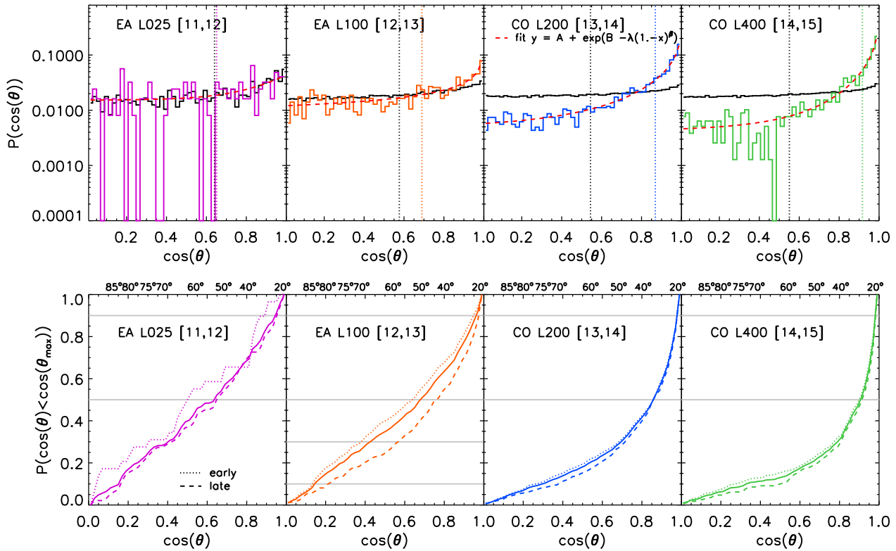
Figure 9. Upper panel: probability distribution function of the cosine of the misalignment angle between the major axis of the distribution of stars inside r_{\text{half}}^{\text{star}} and the major axis of the entire halo for four halo mass bins. The black histograms indicate the probability distributions for the total sample of haloes that satisfies the resolution criteria, whereas coloured histograms refer only to the subsample of haloes whose mass is indicated in the legend. Vertical lines indicate the median values of the misalignment angle (same colour convention as for the histograms). Red dashed curves represent the analytic fit discussed in Appendix B. Lower panel: cumulative version of the probability function for early- and late-type galaxies (dotted and dashed curves respectively).
