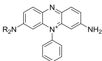
R = H, Phenosafranin R = Et, Methylene violet 3RAX
