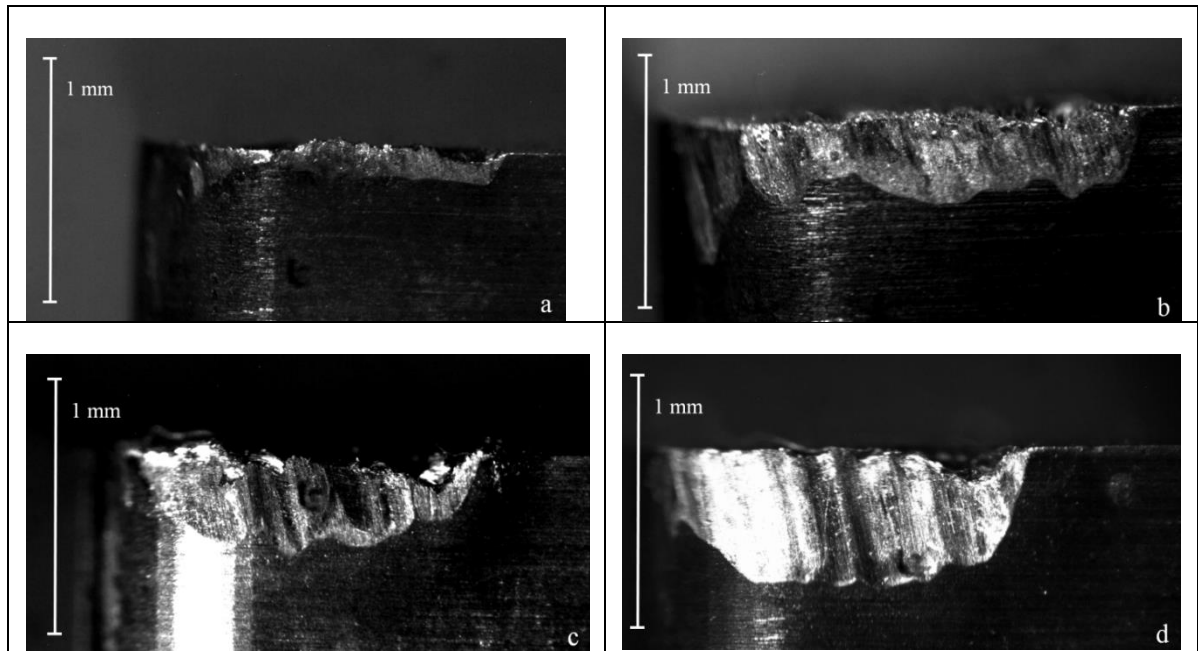
Fig. 8: Wear flat in milling nickel alloy with WC6 cutting inserts coated with: a): TiAlN-ZrNbN-CrN , (FCVAD ); b): Ti-TiAlN-TiN , (FCVAD); c): Ti-TiCrAlN , (standard arc-PVD); d): Ti-TiN , (standard arc-PVD); Machining time – 8 min; v = 40 m/min; a_p = 1.0 mm; f_z = 0.15 mm/tooth
