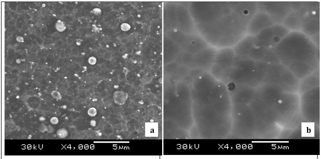
Fig.2. Surface morphology of Ti-TiCrAlN : (a) - standard arc-PVD; (b) - TiAlN-ZrNbN-CrN (FCVAD):
