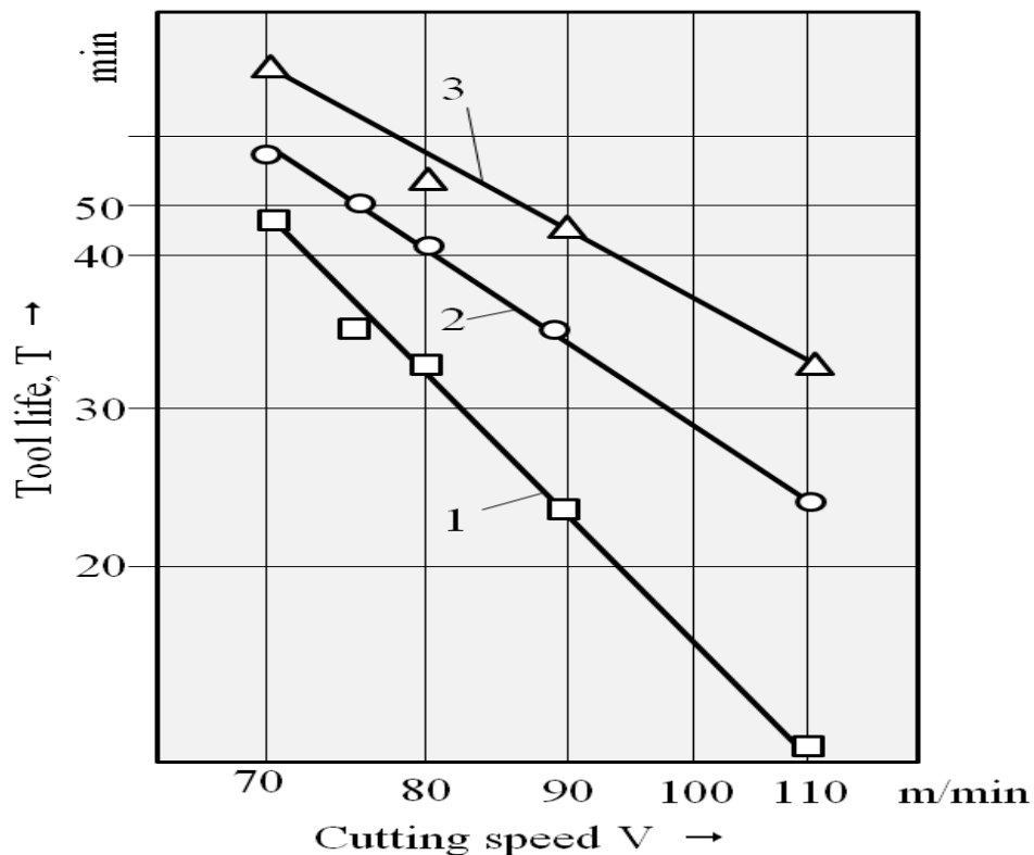
Fig. 4: WC6 tool life as a function of cutting speed in turning titanium alloy for a_p = 1.0\text{ mm} ; f = 0.2\text{ mm/rev} :
