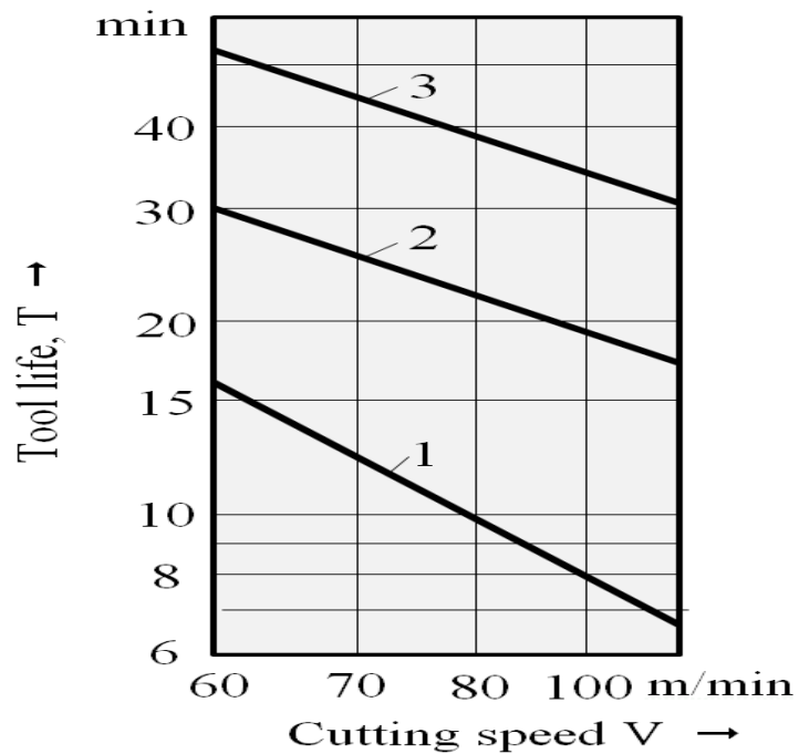
Fig. 6: WC6 tool life as a function of cutting speed in face milling of titanium alloy VT20 for a_p=0,1 mm; f_z=0,1 mm/tooth;
