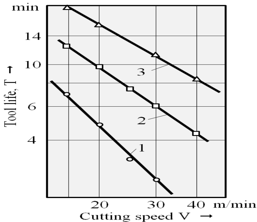
Fig. 7: VK6 tool life as a function of cutting speed in face milling of Ni- alloy for a_p = 1.5 mm; f_z = 0.1 mm/tooth; 1 – uncoated; 2 - Ti-ZrCrAlN coating (standard technology arc-PVD); 3 - TiAlN-ZrNbN-CrN (elaborated technology FCVAD).
