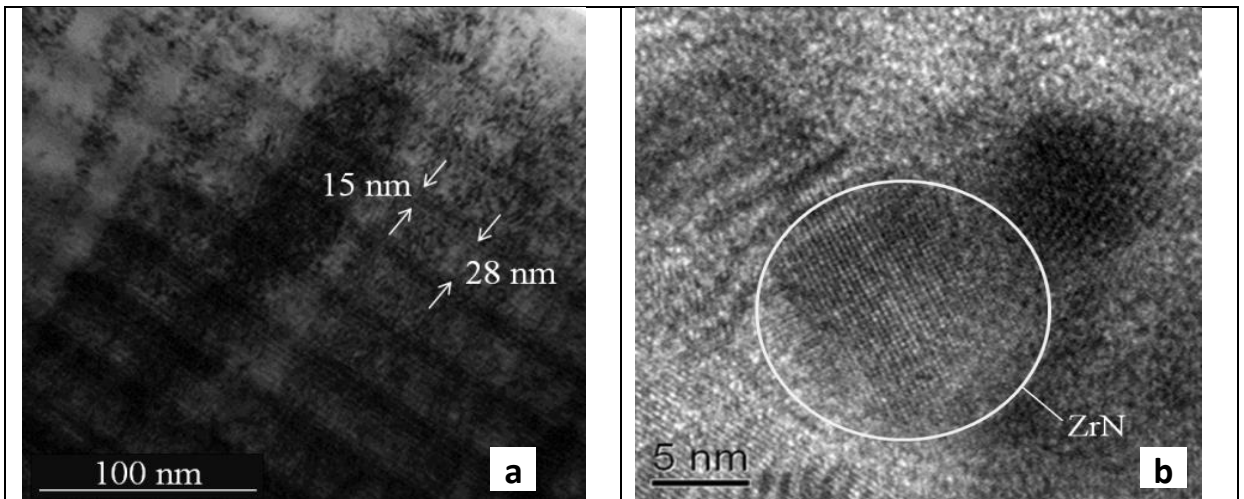
Fig. 3: Cross sectional structure of a TiAlN-ZrNbN-CrN coating :
