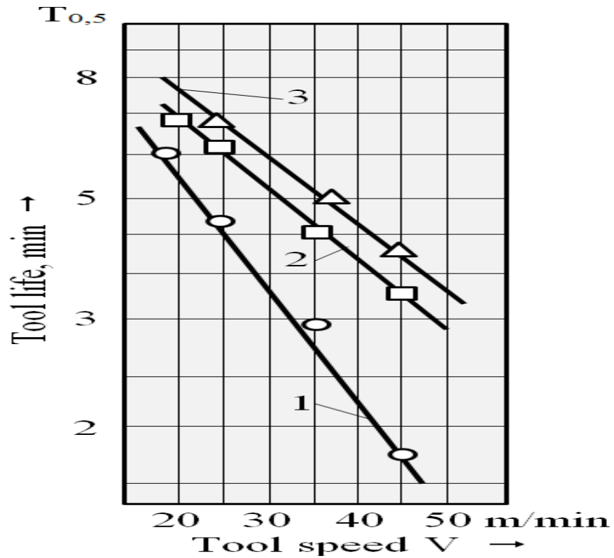
Fig. 5: VK6 tool life as a function of cutting speed in turning nickel alloy CN77TUR for a_p = 0.5 mm; f = 0.15 mm/rev;.
