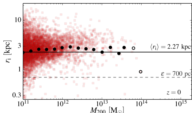
Figure 14. The characteristic radius, r_i , of the central component as function of halo mass (equation 19) for haloes in the EAGLE simulation. The red squares correspond to all the haloes fitted individually and the overlaying black circles to the stacked haloes in each mass bin. Stacks containing less than three objects are shown as open circles. The minimum Plummer-equivalent softening length ( \epsilon = 0.7 kpc) is indicated by the grey dashed line at the bottom of the figure. The average value of the stacks with more than three objects is indicated by a solid black line.
