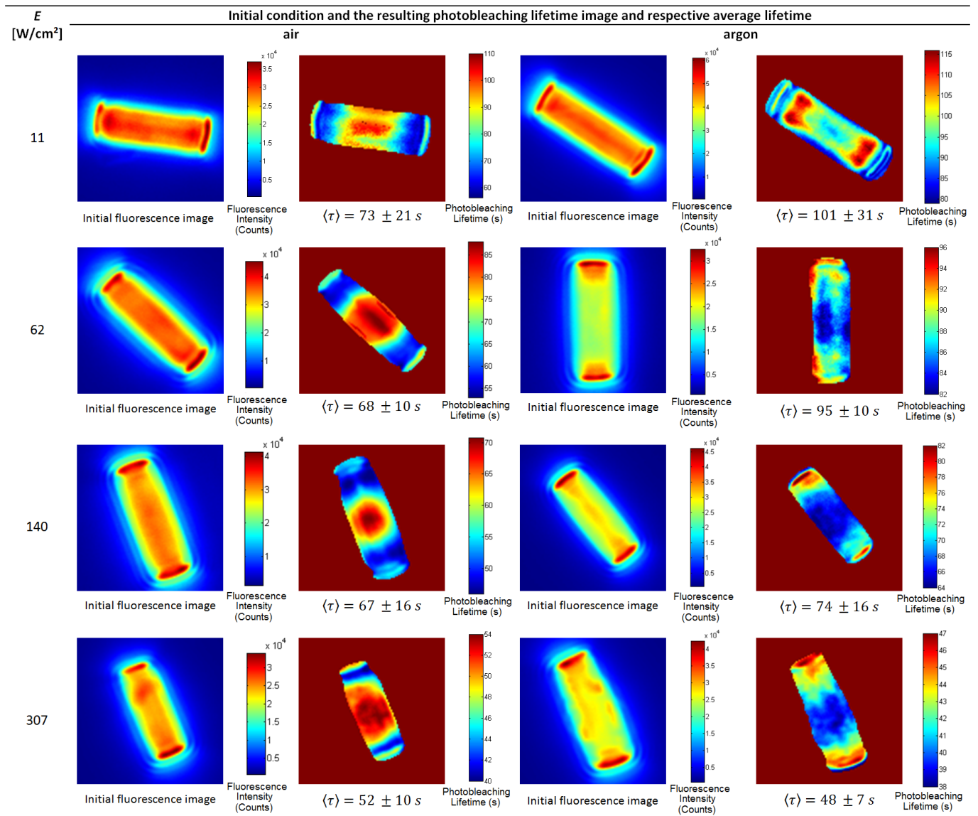
Figure 13 Photobleaching lifetime images of zeolite L hosted with thionine as a function of excitation irradiance in air and in argon atmosphere. For each experimental condition at least ten zeolites were analyzed individually, and the average photobleaching lifetime and its standard deviation are presented. The window of each image represents a square with side of 8.5 \mu\text{m} .
