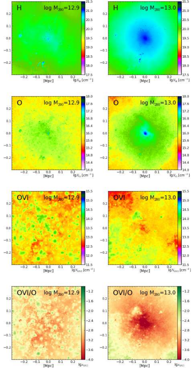
Figure 12. The same group-sized halo (Grp004, M_{200} = 10^{12.89}M_{\odot} ) at z = 0.2 simulated using the standard EAGLE prescription (left) and without AGN feedback model (right) in the same format as Fig. 2. From top-to-bottom, 600 kpc snapshots of hydrogen, oxygen, and O VI columns are shown as well as the O VI ionization fraction. The NoAGN halo has M_{200} = 10^{12.97}M_{\odot} , compared to 10^{12.89}M_{\odot} with AGN feedback due to weaker feedback, but we use a constant R_{200} = 387 kpc when comparing virial quantities.
