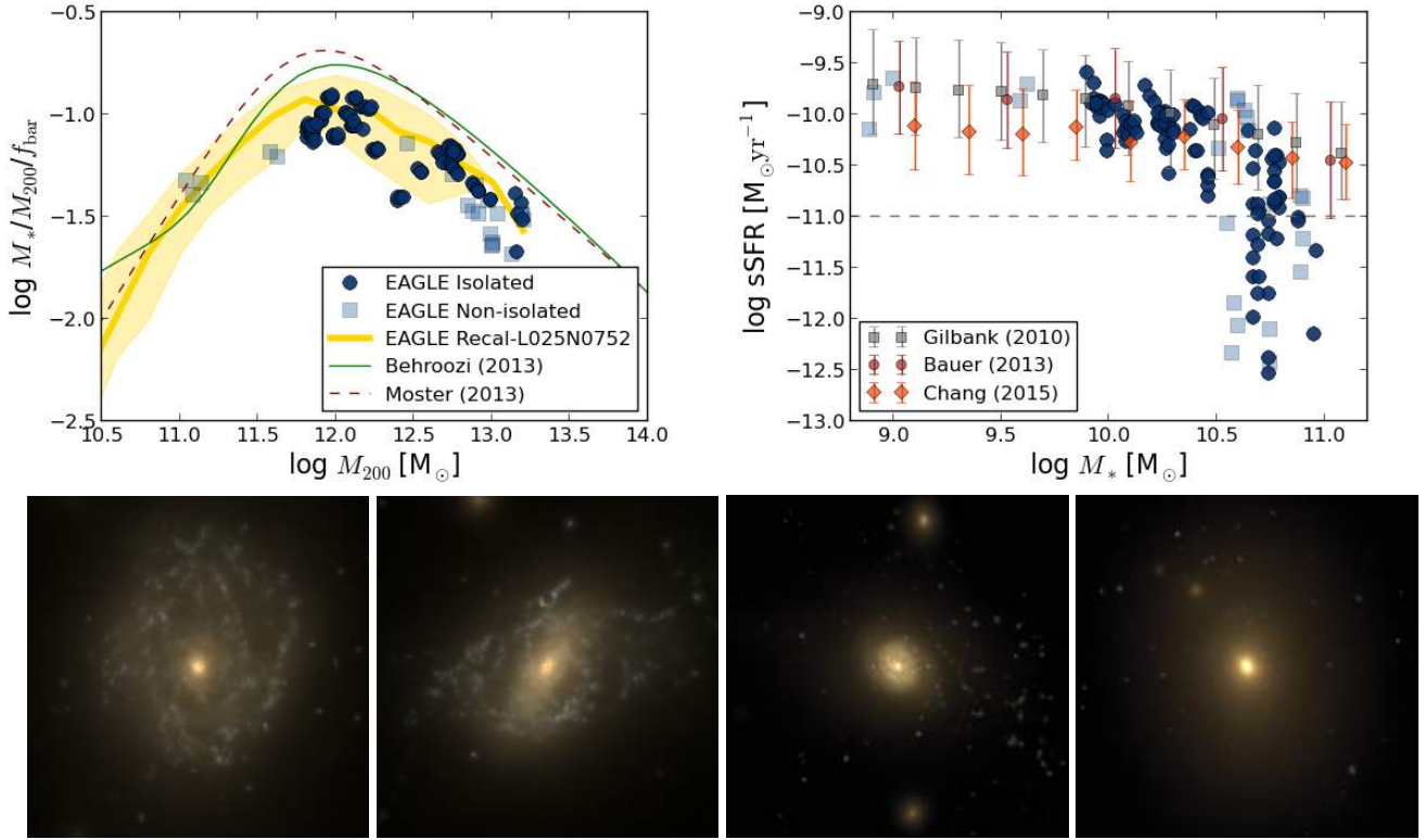
Figure 1. Stellar mass to halo mass ratio plotted as a function of halo mass of zoomed centrals (top left) and sSFR as a function of stellar mass (top right) from 6 redshifts ( z = 0.25 \rightarrow 0 ) that we use in our analysis. Galaxies that can be considered “isolated” by COS-Halos criteria are indicated by dark circles, while transparent squares indicate galaxies with a neighboring galaxy with M_* > 10^{10.3} M_\odot within 300 kpc. Three sub- L^* galaxies at z = 0.205 are also plotted as light circles. The thick yellow line is the fit to all centrals in the Recal-L025N0752 simulation (S15) with the shading indicating the 1\text{-}\sigma dispersion. Abundance matching results from Behroozi et al. (2013, solid green) and Moster et al. (2013, dashed red) at z = 0.2 are displayed on the left, and observations of the sSFR of star-forming galaxies as a function of M_* from Gilbank et al. (2010, grey squares), Bauer et al. (2013, brown circles), and Chang et al. (2015, orange diamonds) are displayed on the right. Bottom panels show simulated 50 kpc SDSS u, g, and r -band composite images, including dust, of two star-forming L^* galaxies and two group centrals—a recent merger and a passive galaxy (from left to right). All plots use M5.3 zooms.
