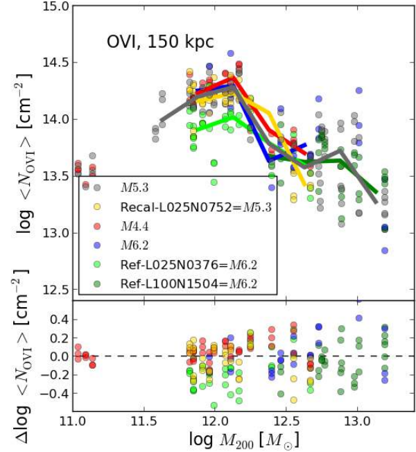
Figure B2. O VI aperture column densities within 150 kpc for our standard NEQ runs at z = 0.205 for the same runs as shown in Fig. B1, showing a range of 64 (4) in mass (spatial) resolution. The aperture is centred on the galaxy coordinates given in each respective simulation (zoom and EAGLE volume). The top panel shows the absolute values (circles) and binned averages (thick lines), and the bottom panel shows differences relative to the M5.3 zooms (grey circles in top panel).
