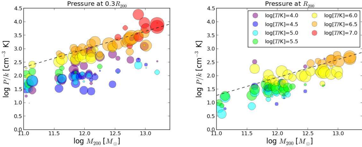
Figure 11. Pressure as a function of halo mass in shells at 0.3\times (left panel) and 1.0\times R_{200} (right panel). Pressures are calculated at a given radius and temperature by multiplying the median density within an 0.1 dex spread in r and T . The dashed lines indicate the pressure of an isothermal density profile at the virial temperature normalized to contain the entire baryonic content of a halo within R_{200} . The symbol areas scale in proportion to the logarithm of the mass, m , contained in this phase normalized to halo mass and radius, such that \text{area} \propto \log[(m/M_{200})(r/R_{200})^{-2}] .
