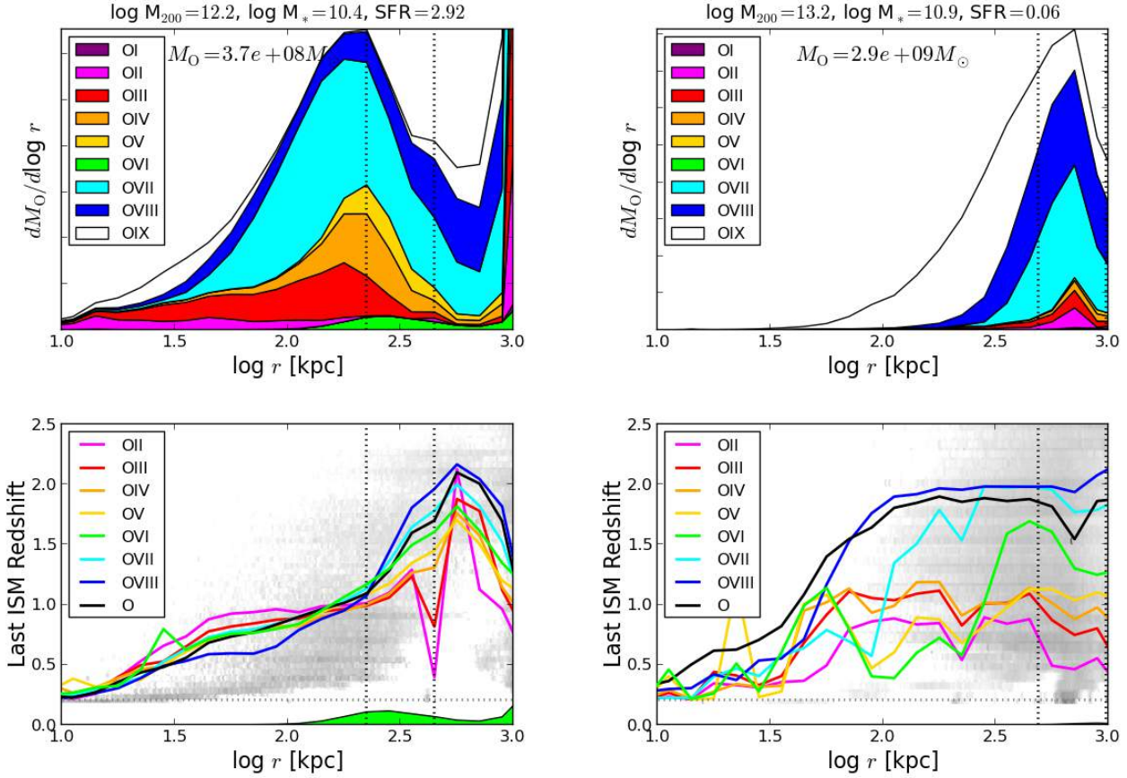
Figure 6. CGM oxygen as a function of radius is plotted in the top panels for the Gal005 L^* halo (left, M_{200} = 10^{12.2}M_{\odot} ) and the Grp008 group-sized halo (right, M_{200} = 10^{13.2}M_{\odot} ). The top solid line indicates the total oxygen content as a function of radius on a linear scale (y-axis values not specified). The total CGM oxygen content in each panel between 10^{1.05} - 10^{2.95} kpc is 3.7 \times 10^8 and 2.9 \times 10^9 M_{\odot} for the L^* and group haloes respectively (listed on the top of each panel). The dotted vertical lines indicate R_{200} and 2R_{200} . The bottom panels indicate the age distribution of oxygen in gray shading, where we define age as the last redshift a SPH particle was in the ISM. The mean ages of oxygen species (coloured lines) and total oxygen (black line) are also shown. The gray horizontal dotted line is the redshift of the snapshot. We also repeat the O VI shading from the top panels in the age panels. O VI in L^* haloes primarily resides outside R_{200} and is greater than 5 Gyr old ( z > 1 ). Group-sized haloes enrich a more extended region at earlier times ( z \sim 2 ).
