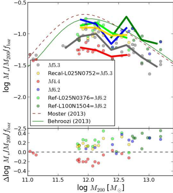
Figure B1. Galaxy formation efficiency as a function of halo mass for our standard NEQ runs at z = 0.205 (in grey) and for matched haloes in Recal-L025N0752 (yellow) at the same resolution ( M5.3 ), the higher resolution M4.4 zooms (red), and the lower resolution M6.2 zooms (blue). We also compare to the matched haloes in Ref-L025N0376 (green) and Ref-L100N1504 (dark green). The outputs for EAGLE volumes are at z = 0.187 , and the abundance matching constraints from Behroozi et al. (2013, solid green) and Moster et al. (2013, dashed red) are at z = 0.2 . The top panel shows the absolute values (circles) and binned averages (thick lines), and the bottom panel shows differences relative to the M5.3 zooms (grey circles in top panel).
