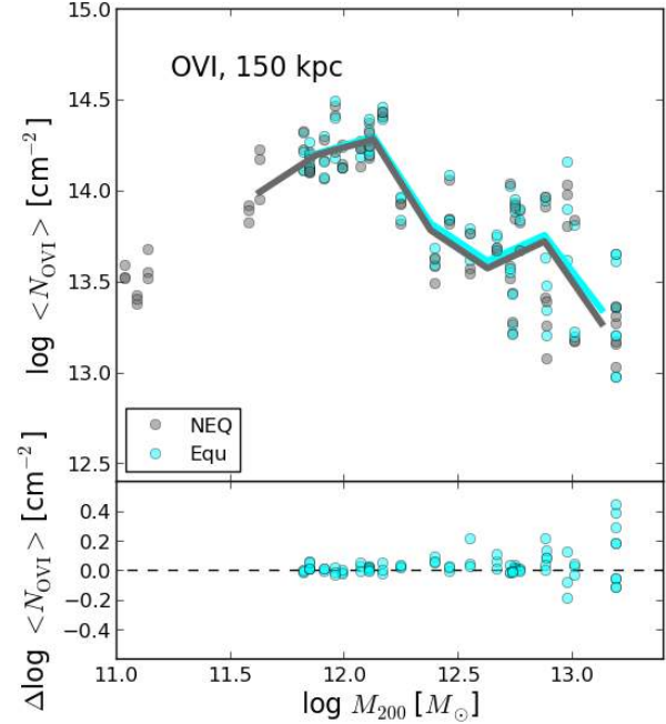
Figure A1. O VI aperture column densities within 150 kpc for our standard NEQ runs at z = 0.205 (grey, a repeat of the left panel of Fig. 4), and runs with equilibrium ionization and cooling (cyan) with the differences relative to the standard NEQ runs shown on the bottom panel (for each halo there are 3 circles corresponding to 3 projections). Thick lines of the same colour in the top panel are binned averages. The runs diverge at z = 0.503 for L^* haloes and z = 0.282 for all but one group halo when the NEQ module is activated for the NEQ runs. Except for some high-mass haloes, the differences are small.
