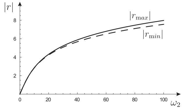
Fig. 11. Attenuation coefficient |r| versus frequency \omega_2 for \beta = 0 + n\pi/3 ( |r_{\min}| ) and \beta = \pi/6 + n\pi/3 ( |r_{\max}| ). The curves are given for \epsilon = 0.1 .
