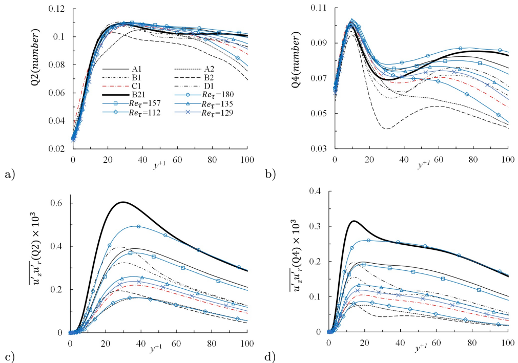
FIGURE 24. Quadrant analysis. (a) Number of ejections (Q2) over the total number of events; (b) Number of sweeps (Q4) over the total number of events; (c) Contributions of ejection (Q2) events to \overline{u'_z u'_r} ; (d) Contributions of sweep (Q4) events to \overline{u'_z u'_r} .
