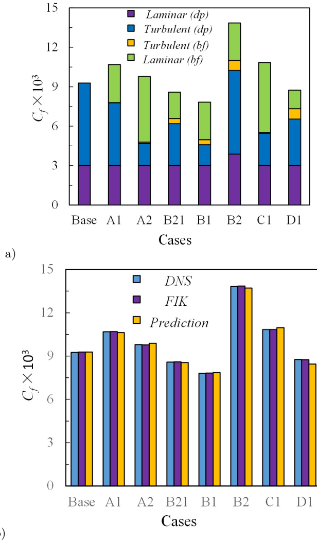
FIGURE 18. Friction coefficient. (a) Contributions of the various components of FIK analysis, Laminar ( dp & bf ) refer to the RHS terms 1 & 3 of equation 3.9, respectively; turbulent ( dp & bf ) refer to the RHS terms 1 & 2 of equation 3.10, respectively; (b) Comparison of friction coefficients calculated from velocity gradient (DNS), FIK analysis and predictions based on EPG reference flows.
