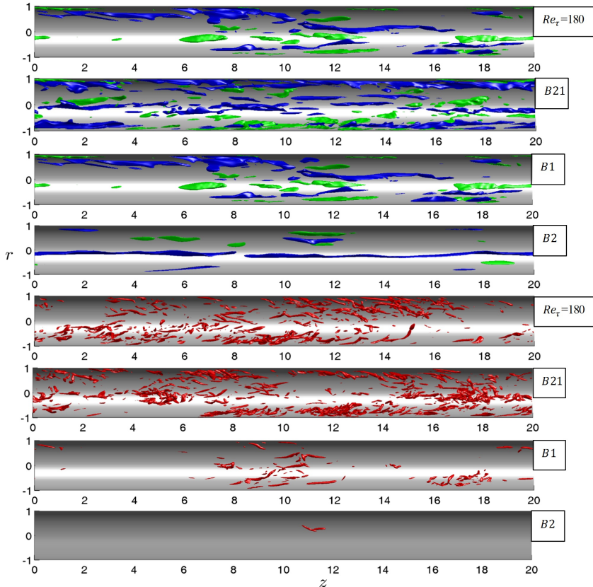
FIGURE 19. Turbulent structures in cases Base, B21, B1 & B2. (a) Top four blocks: High (green) and low (blue) speed streaks illustrated with 3D iso-surfaces of u'_z = \pm 0.15 and (b) Bottom four blocks: vortical structures illustrated with 3D iso-surfaces of \lambda_2 = -1.0 .
