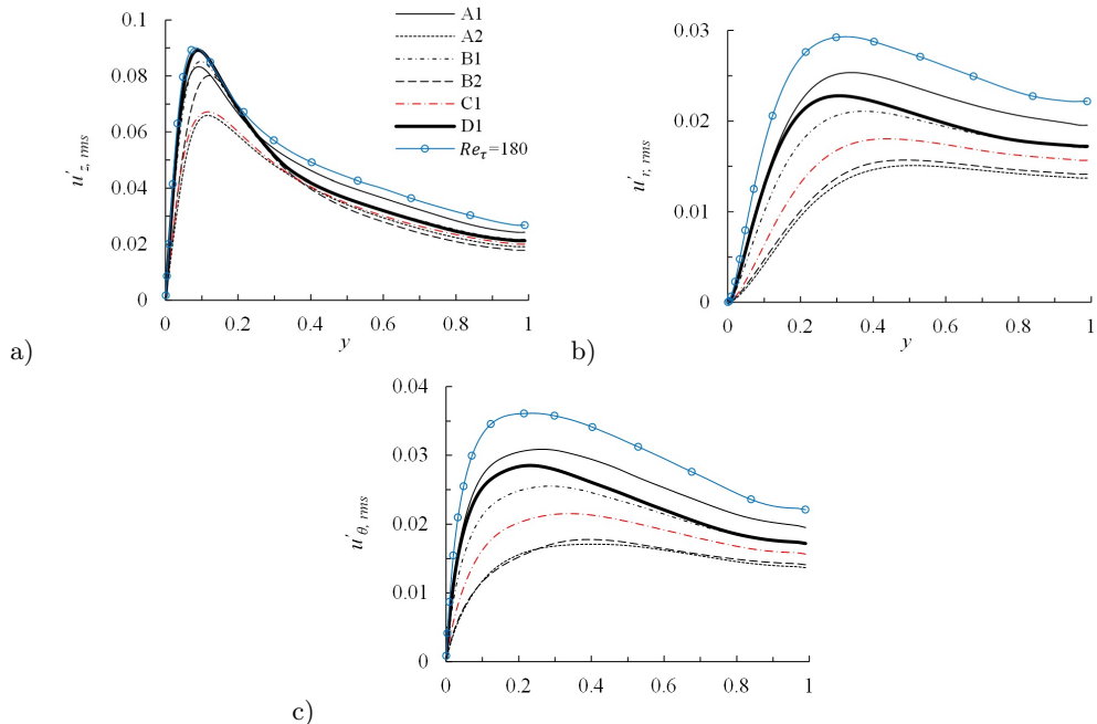
FIGURE 7. Distribution of the root-mean-square of the turbulent velocities.
