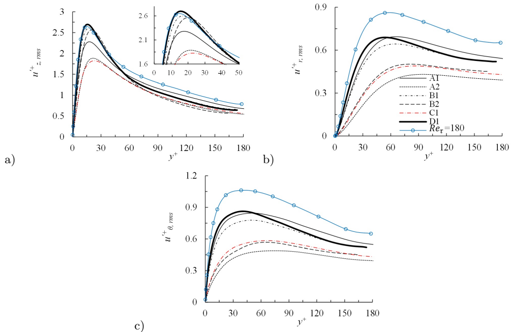
FIGURE 8. Distribution of the root-mean-square of the turbulent velocities in wall units.
