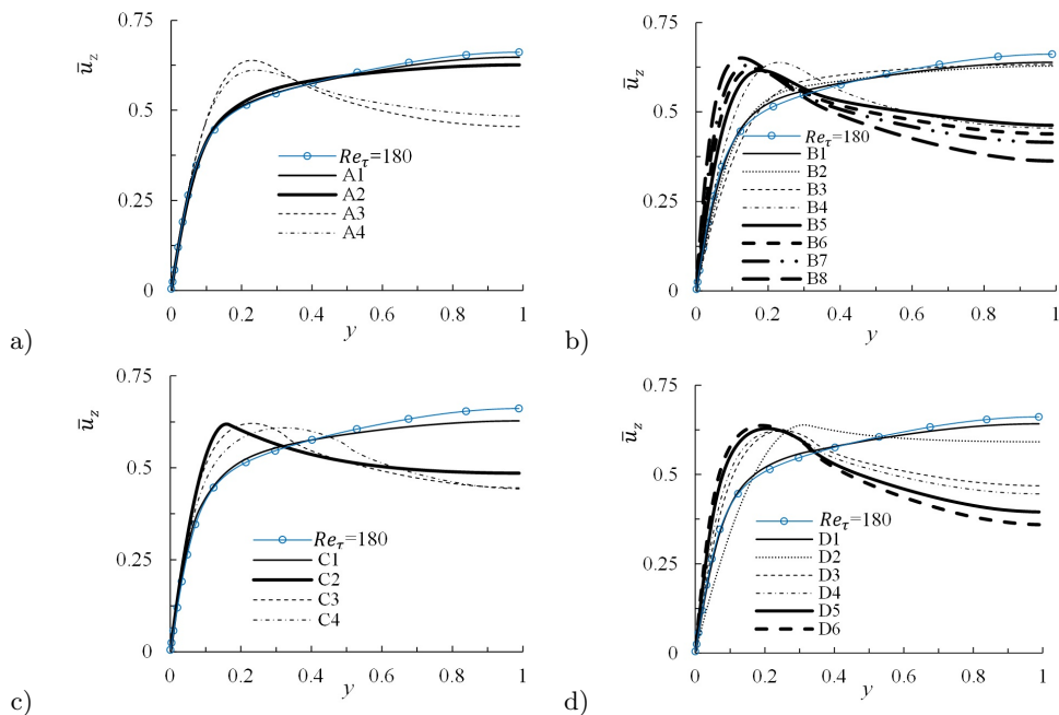
FIGURE 3. Mean velocity profiles of all test cases.
