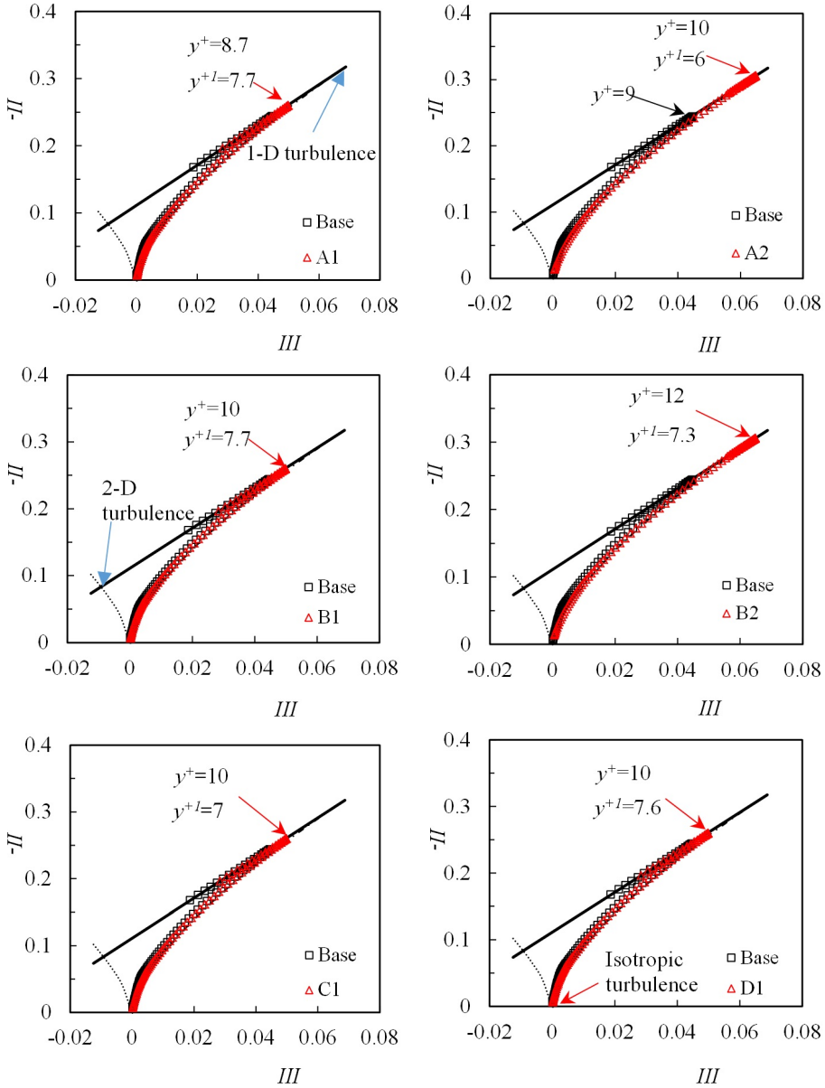
FIGURE 25. The anisotropic invariant maps (AIM) of a number of flow cases.
