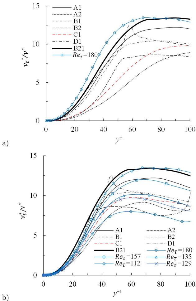
FIGURE 10. Distribution of turbulent viscosity in wall distance based on (a) conventional friction velocity and (b) apparent friction velocity.
