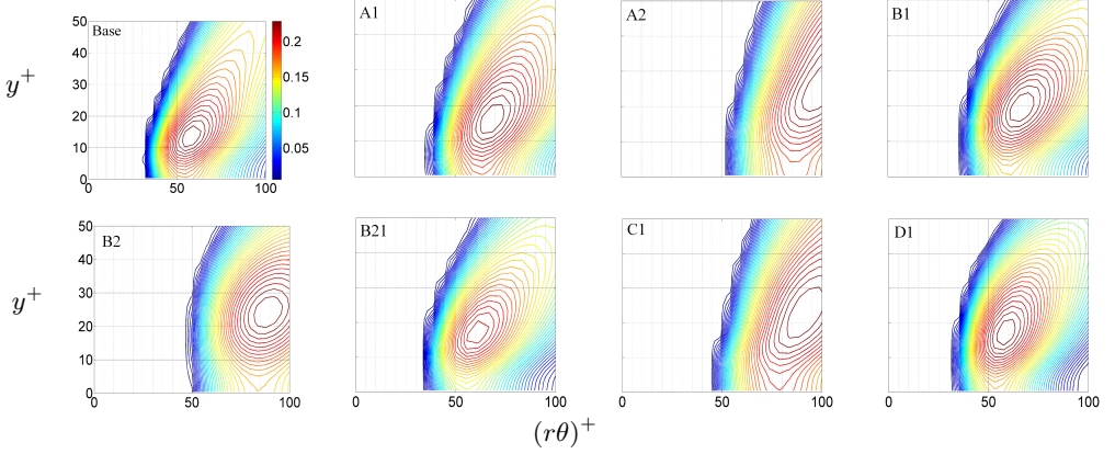
FIGURE 22. Contours of the streamwise velocity correlations in a vertical plane in wall units based on the conventional friction velocity.
