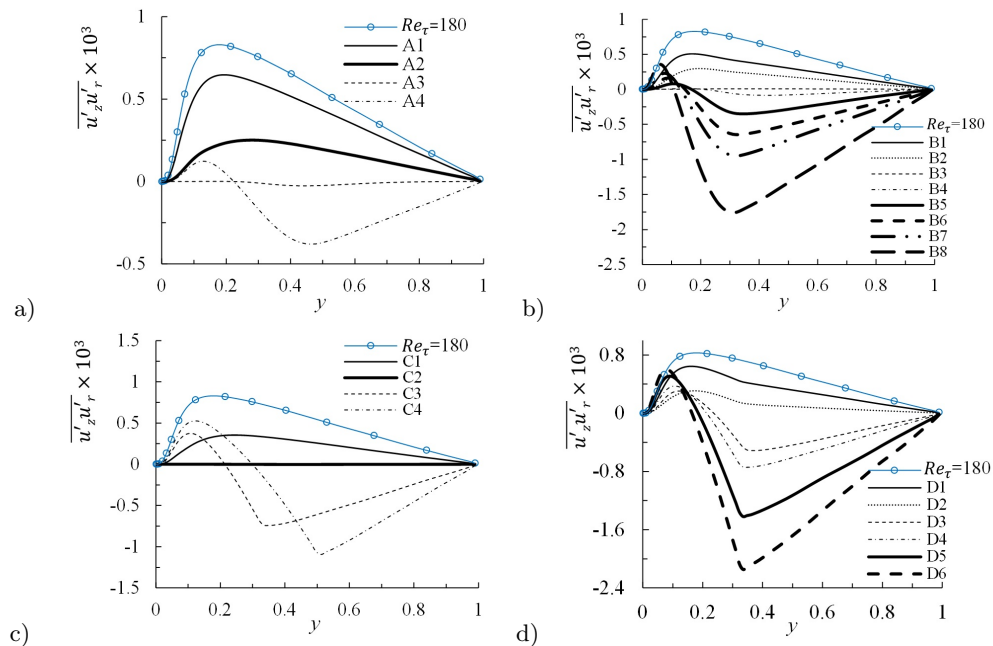
FIGURE 5. Distribution of turbulent shear stress in all test cases.
