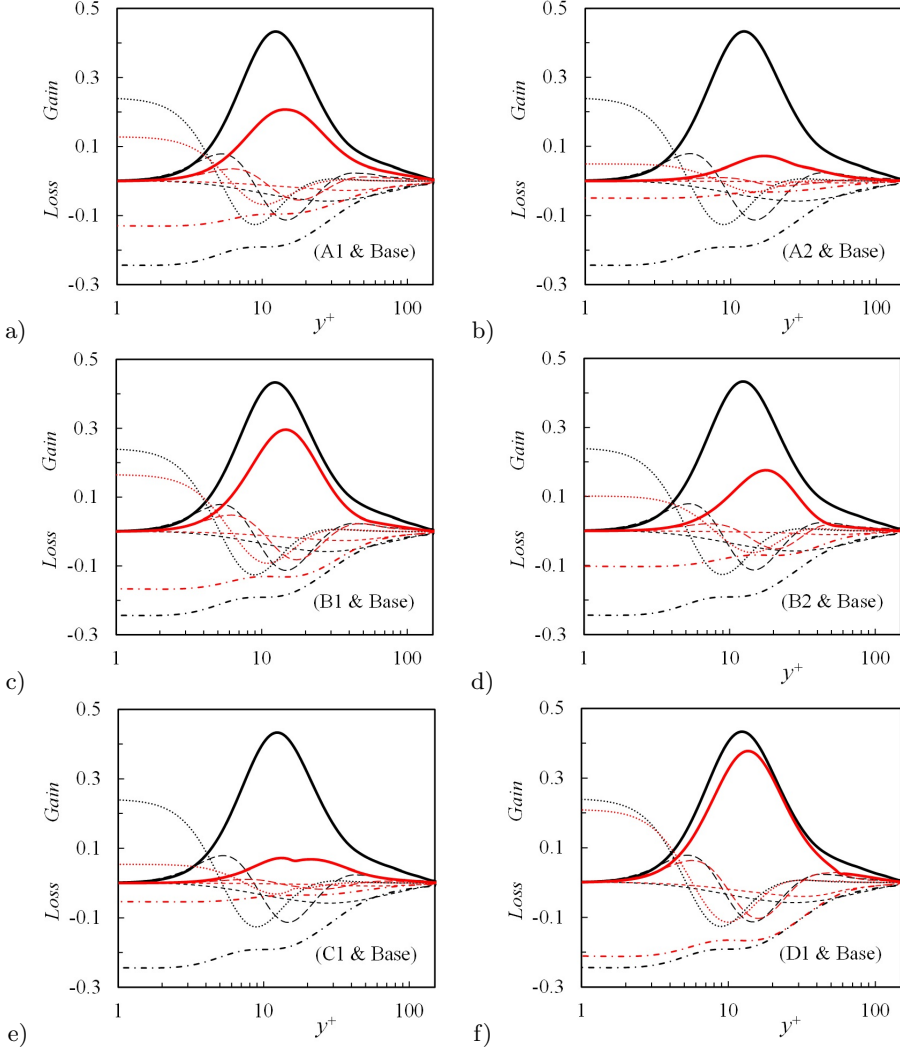
FIGURE 13. The budget terms of the streamwise turbulent fluctuating velocity in conventional wall units. Solid lines: production; Chain dotted lines: dissipation; Short dash lines: pressure strain; Long dash lines: turbulent transport; Dot lines: viscous diffusion. Thick lines: base case ( Re_\tau = 180 ); Thin lines: body-force influenced cases.
