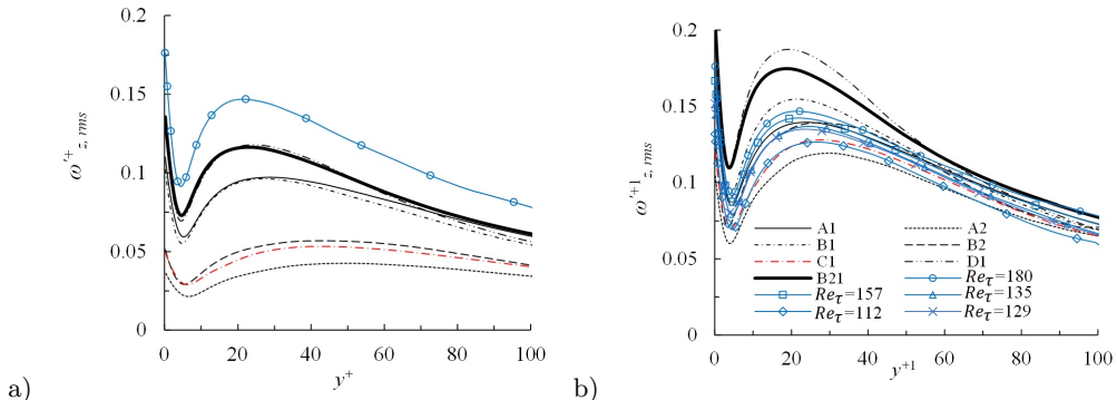
FIGURE 21. Root-mean-square of streamwise vorticity fluctuations normalised using the (a) conventional friction velocity (b) apparent friction velocity.
