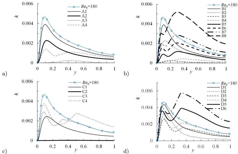
FIGURE 6. Distribution of turbulent kinetic energy in all test cases.
