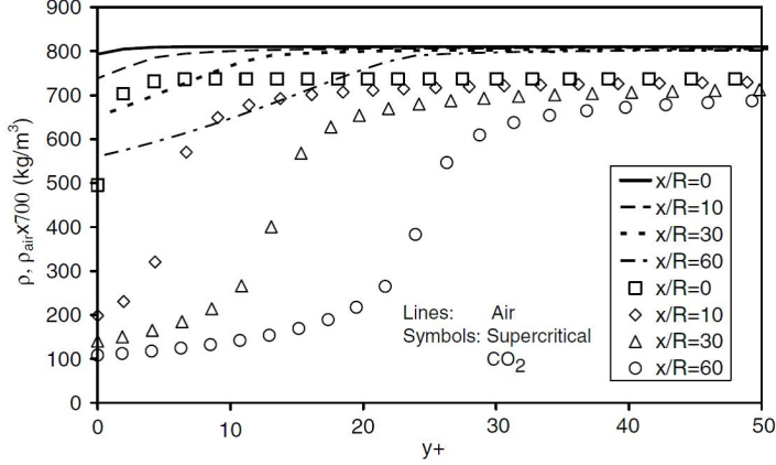
FIGURE 1. Examples of distributions of density in mixed convection of a flow of an air and \text{CO}_2 at supercritical pressure. ‘ x/R ’ is the distance from the start of the heated length of the pipe over radius. (Reproduced from He et al. (2008) with permission)
