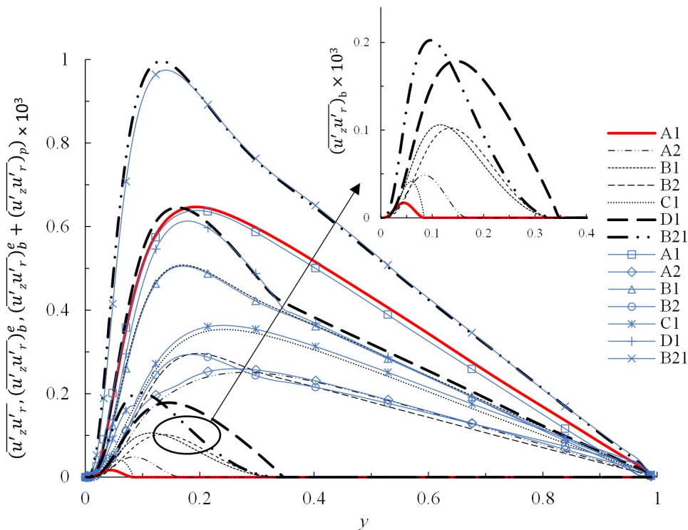
FIGURE 11. Distribution of turbulent shear stresses, (i) DNS results \overline{u'_z u'_r} (lines only in main figure), (ii) Estimated turbulent shear stress due to body force calculated from equation 3.7, \overline{(u'_z u'_r)_b} , (lines only in inset) and (iii) Estimated overall turbulent shear stress using EPG reference flow data, \overline{(u'_z u'_r)_p} + \overline{(u'_z u'_r)_b} , (lines with markers).
