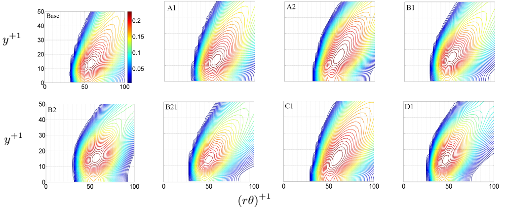
FIGURE 23. Contours of the streamwise velocity correlations in a vertical plane in wall units based on an apparent friction velocity.
