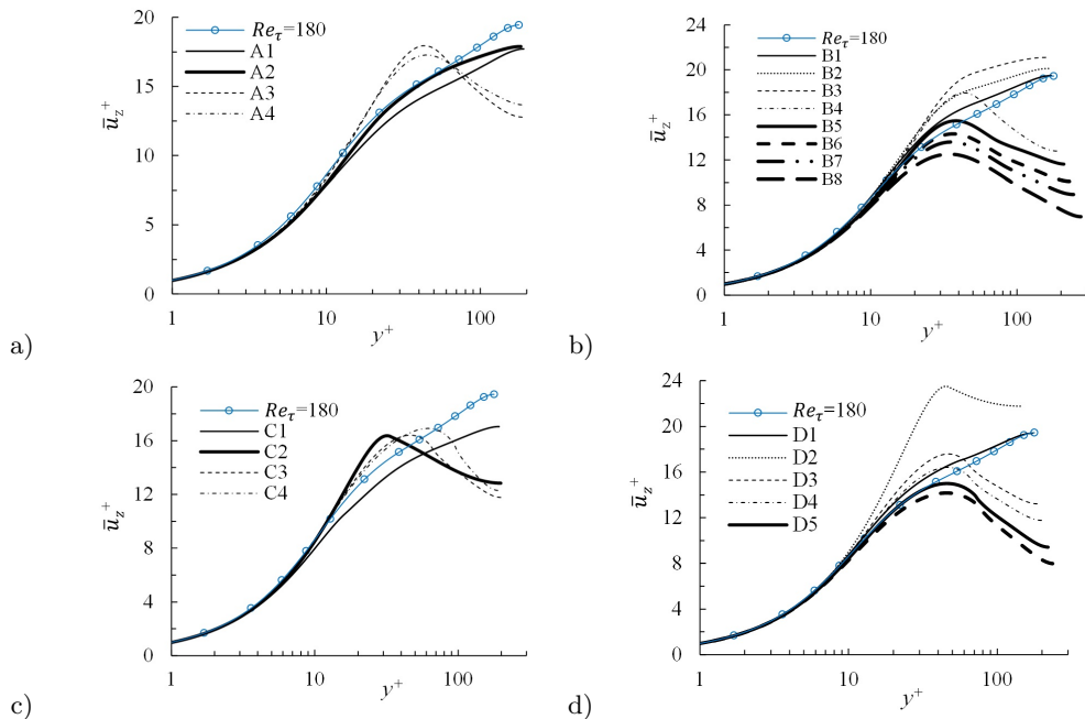
FIGURE 4. Mean velocity profiles of all test cases in wall coordinates.
