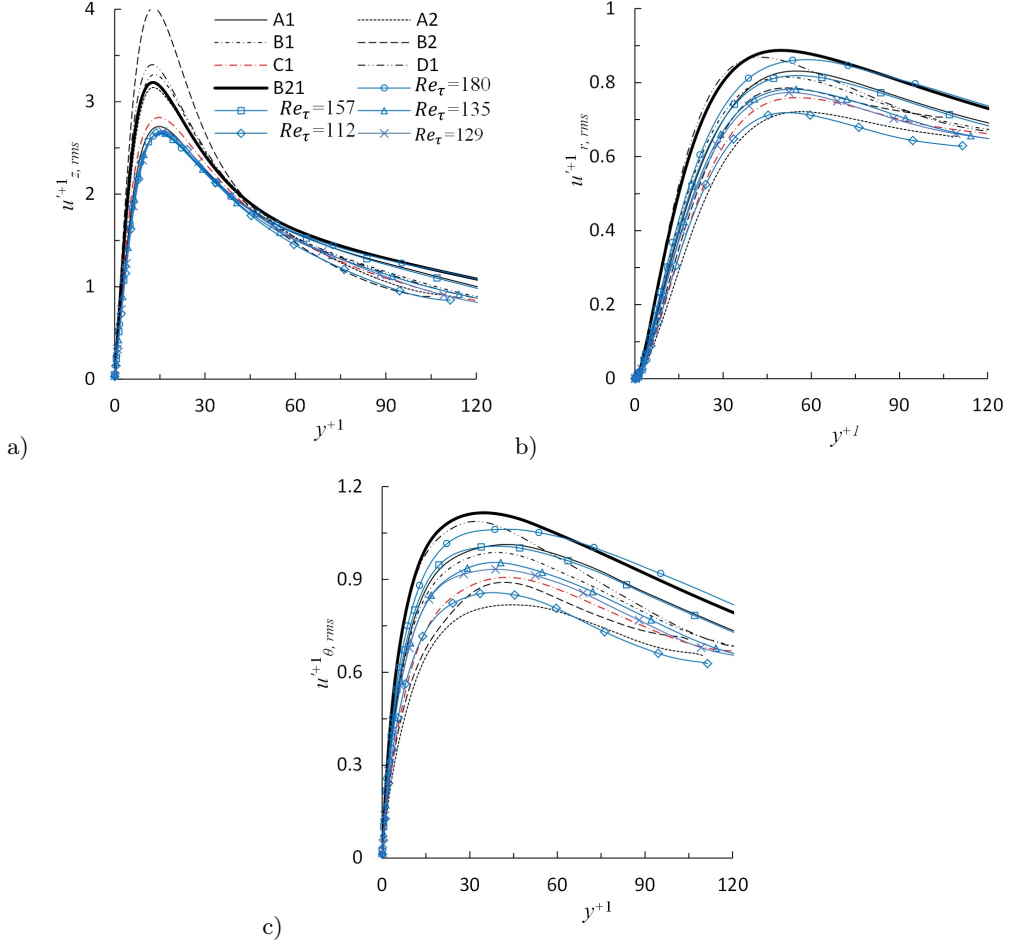
FIGURE 12. Distribution of the root-mean-square of turbulent velocities normalised by the apparent friction velocity.
