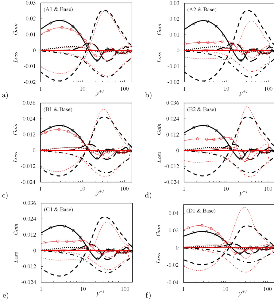
FIGURE 16. The budget terms of the wall-normal turbulent fluctuating velocity in wall units based on the apparent friction velocity. See figure 14 for legend.
