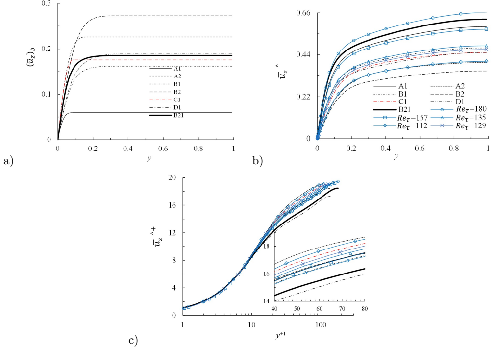
FIGURE 17. Velocity profiles. (a) Body-force induced perturbation flow; (b) Total flow subtracting the body-force induced flow, together with EPG reference flows; and (c) Same as (b) but in wall coordinates.
