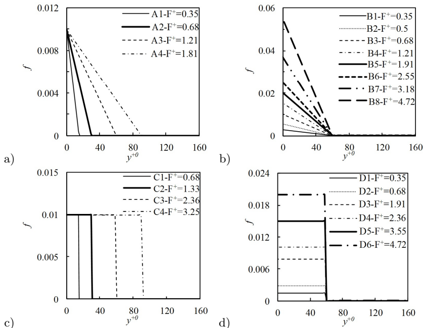
FIGURE 2. Body force distributions ( y^{+0} = y^* u_{\tau_0}^* / \nu^* , F^+ = F^* / (2\tau_w^* R^*) where u_{\tau_0}^* and \tau_w^* are the friction velocity and the wall shear stress of the base flow, Re_\tau = 180 , respectively).
