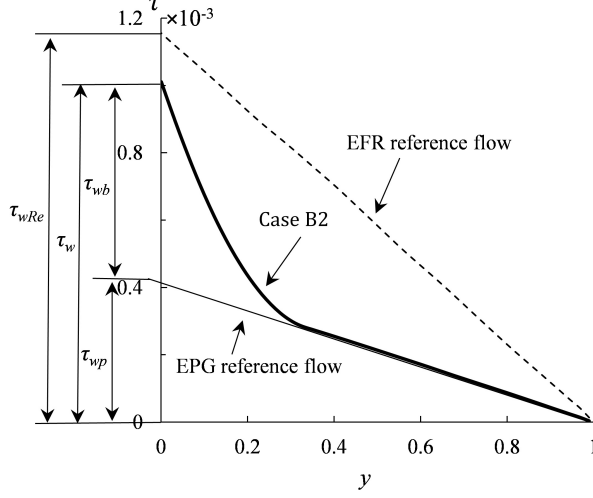
FIGURE 9. Total and wall shear stresses of case B2 and those of its corresponding EFR and EPG reference flows.
