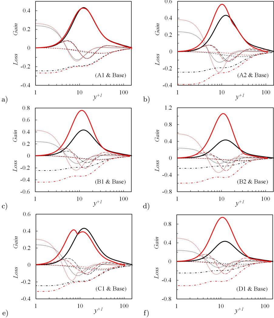
FIGURE 15. The budget terms of the streamwise turbulent fluctuating velocity in wall units based on the apparent friction velocity. See figure 13 for legend.
