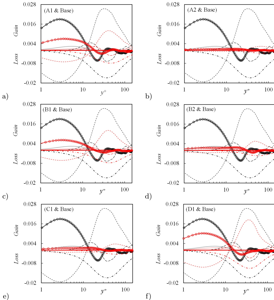
FIGURE 14. The budget terms of the wall-normal turbulent fluctuating velocity in conventional wall units. Solid lines with markers: pressure diffusion; Chain dotted lines: dissipation; Short dash lines: pressure strain; Long dash lines: turbulent transport; Dot lines: viscous diffusion. Thick lines: base case ( Re_\tau = 180 ); Thin lines: body-force influenced cases.
