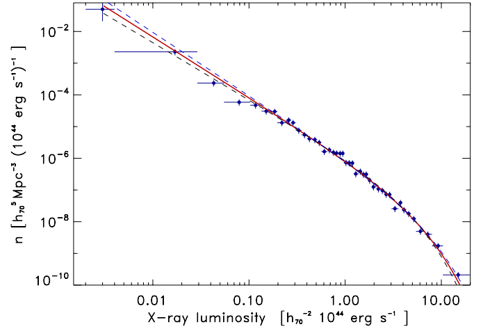
Fig. 1. REFLEX II X-ray luminosity function for the redshift range z = 0-0.4 . We also show the best fitting Schechter function and two bracketing solutions indicating the estimated uncertainties.
