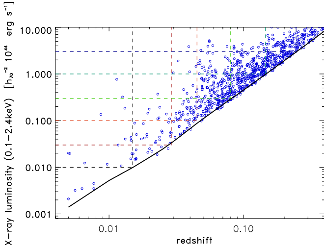
Fig. 2. Median lower detection limit for the X-ray luminosity as a function of redshift in the flux-limited REFLEX II survey (black line). The data points show the luminosity and redshift distribution of the individual REFLEX II clusters. We also show the limits of six volume-limited subsamples of the REFLEX II survey used to assess the density distribution in this paper.
