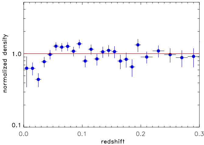
Fig. 3. Cluster density distribution as a function of redshift for the REFLEX II galaxy clusters for a minimum luminosity of 10^{42} erg s ^{-1} (0.1–2.4 keV). The density distribution has been normalised by the predicted redshift distribution as explained in the text.
