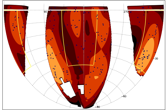
Fig. 7. Cluster density distribution of REFLEX II galaxy clusters in the redshift shell z = 0.0 – 0.06 shown in equatorial coordinates. The density distribution was smoothed by a Gaussian kernel with \sigma = 10 deg, normalised to an integral of 1. The colour scale for the density ratio compared to the mean is defined by orange \geq 2 , light red = 1–2, brown = 0.5–1, dark brown \leq 0.5 . The regions of the Magellanic Clouds are excised from the REFLEX II Survey and the galaxy survey regions of Whitbourn & Shanks (2014) are indicated by yellow solid lines.
