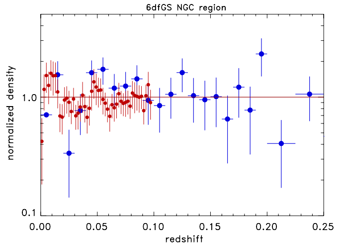
Fig. 9. REFLEX II cluster density distribution as a function of redshift for the region RA = 150–220° and Dec = –40–0° in the north Galactic cap for the same luminosity limit as in Fig. 8. The density distribution has been corrected by means of the survey selection function and normalised to unity. The region corresponds to region 6dFSG-NGC of Whitbourn & Shanks (2014). We also show the results of their assessment of the galaxy distribution out to z = 0.1 in this region with small red data points.
