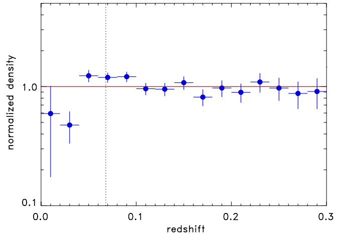
Fig. 5. Cluster density distribution as a function of redshift for the REFLEX II galaxy clusters for a minimum luminosity of 0.2 \times 10^{44} erg s ^{-1} (0.1–2.4 keV). The density distribution has been normalised by the predicted redshift distribution as explained in the text. The vertical dotted line shows the redshift range up to which the sample is essentially volume-limited.
