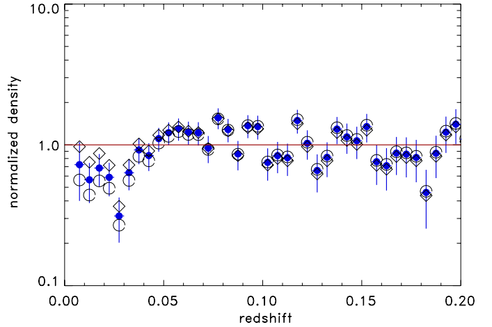
Fig. 4. Cluster density distribution as a function of redshift for the REFLEX II galaxy clusters for a minimum luminosity of 10^{42} erg s ^{-1} (0.1–2.4 keV). Same as Fig. 3, adding the results for using the bracketing X-ray luminosity functions: low bias (open diamonds) and high bias (open circles).
