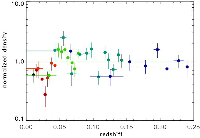
Fig. 6. Relative density distribution of the REFLEX II clusters represented by six volume-limited subsamples as a function of redshift. The relative normalisation of the subsamples has been determined from Eq. (1) as explained in the text.
