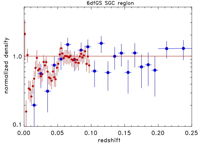
Fig. 8. REFLEX II cluster density distribution as a function of redshift for the region RA = 0–50, 330–360° and Dec = –50–0° in the south Galactic cap for a minimum luminosity of 0.2 \times 10^{44} erg s -1 (0.1–2.4 keV). The density distribution has been corrected by means of the survey selection function and normalised to unity. The region corresponds to region 6dFSG-SGC of Whitbourn & Shanks (2014). We also show the results of their assessment of the galaxy distribution out to z = 0.1 in this region with small red data points.
