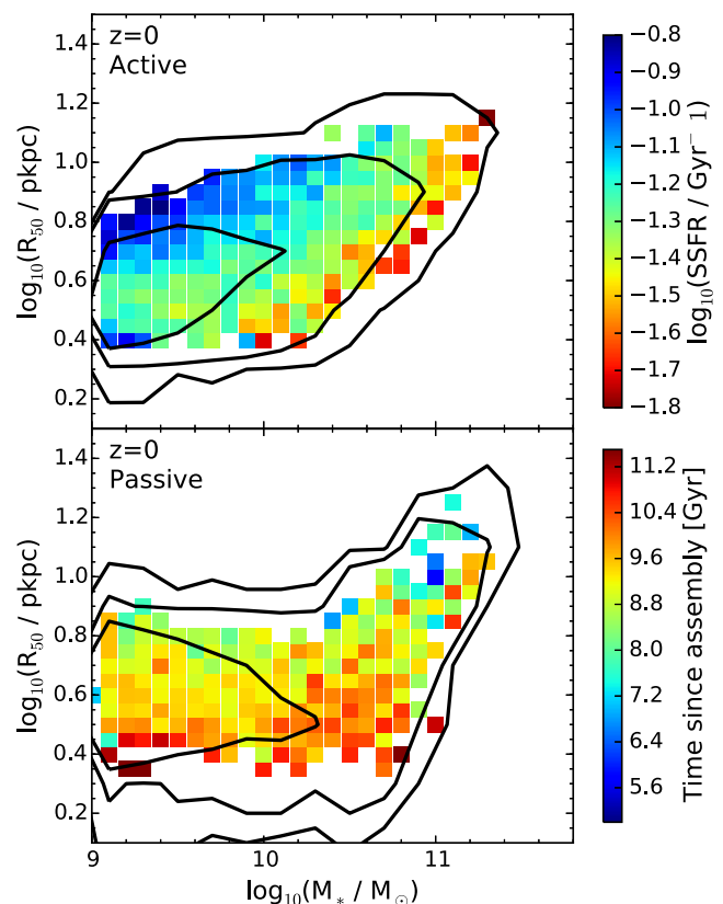
Figure 2. The z = 0 size–mass relations for active and passive galaxies are shown in the top and bottom panels respectively. Black contours indicate the 1, 2 and 3 sigma levels. The galaxy sizes and stellar masses are binned, with each point coloured by the median SSFR for active galaxies (upper panel) or the time since the main progenitor reached half its present-day stellar mass for passive galaxies (lower panel). There is a clear correlation between the scatter in the size–mass relation and these properties.
