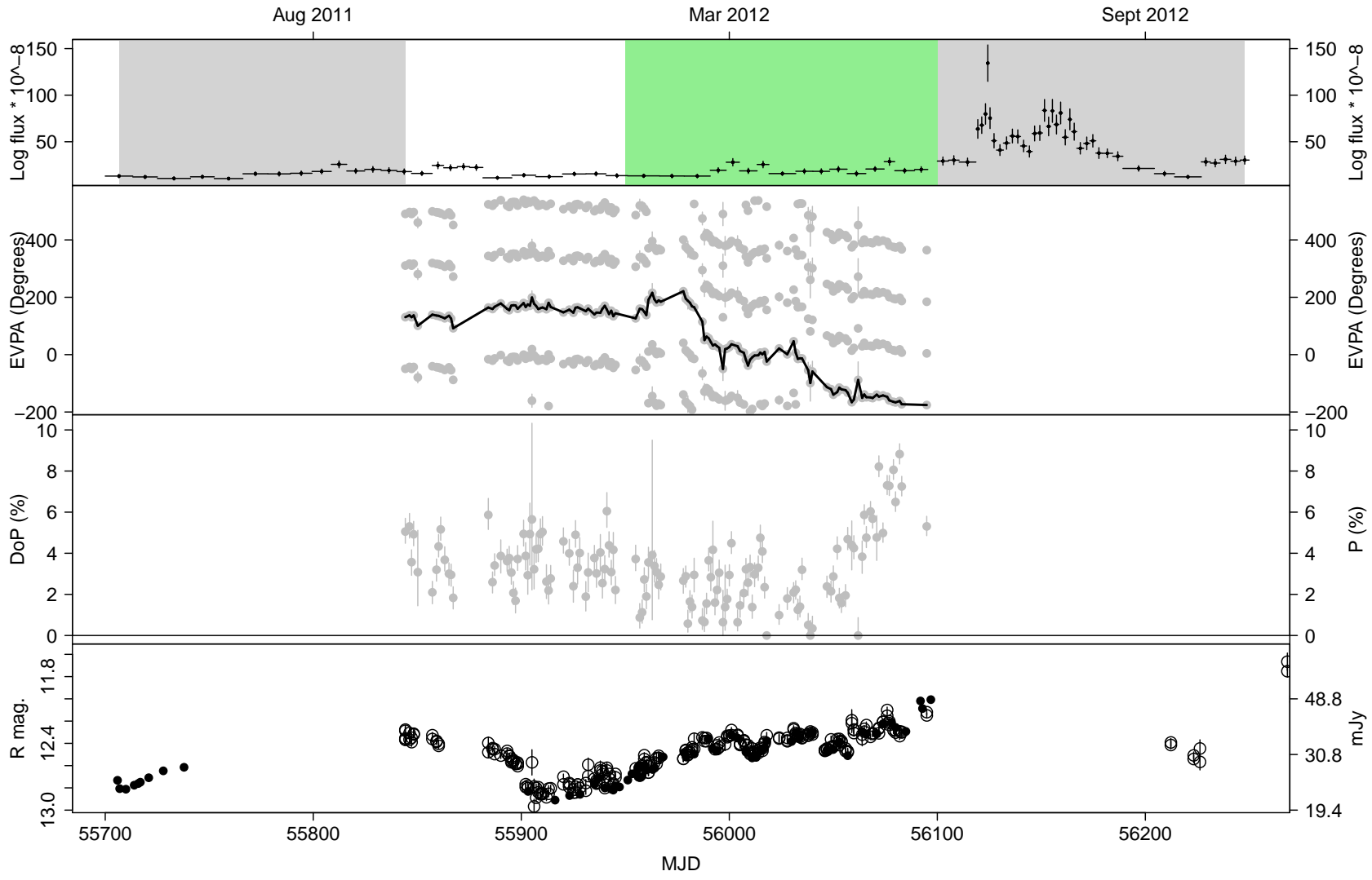
Figure 15. All \gamma -ray and optical data for 3Mrk 421. Top panel shows the Fermi \gamma -ray light curve. The errors on the x axis represent the bins used for the Fermi data. Grey vertical sections show periods where no synchronous optical data available, the green vertical section highlights the region where the optical polarisation angle rotates in the downwards direction. Flaring episodes are identified by vertical blue lines (see Section 2.3.1 for definition of a flare). The second panel shows the optical polarisation angle or electric vector position angle (EVPA), the grey points are RINGO2 data and no KVA-DIPOL data are available. The black line traces the temporally closest EVPA points, showing the most likely behaviour of the EVPA. The third panel shows the optical degree of polarisation (again no KVA-DIPOL data are available), and the fourth panel shows the optical magnitude; photometric calibration of the RINGO2 data was not possible due to the lack of suitable secondary stars in the frame, we instead present SkyCamZ data (open circles) to complement the KVA-DIPOL data.
