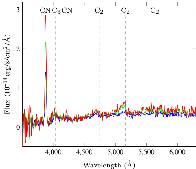
Figure 5. Sky-subtracted spectra of comet 67P obtained on September 5 with LOTUS. The spectra are extracted at three different apertures centred on the comet nucleus with diameters 8.4" (blue line), 16.8" (green line) and 33.6" (red line).
