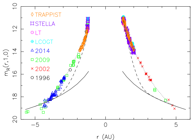
Figure 3. Total R -band magnitude within \rho = 10,000 km, corrected to unit geocentric distance and zero degrees phase angle, against heliocentric distance. The solid line shows the predicted magnitude of the inactive nucleus, the dashed line a prediction based on the expected total water prediction rate, and the dotted line an empirical prediction based on photometry from previous orbits (see Snodgrass et al. 2013, for details)
