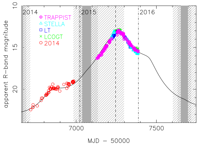
Figure 1. Prediction vs measurements of total R -band magnitude within \rho = 10,000 km. Hatched, cross hatched and solid shading shows periods when the solar elongation is less than 50, 30 and 15 degrees respectively. The vertical dashed line marks perihelion.
