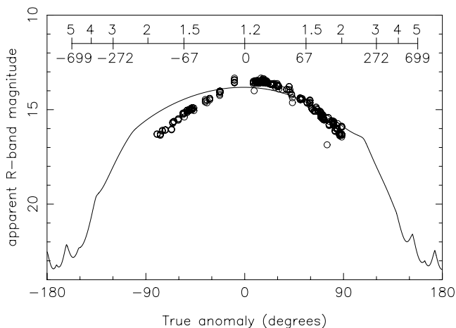
Figure 7. Comparison of photometry (within \rho = 5'' aperture) with simple thermophysical model. The upper bar shows r and \Delta T (in AU and days, respectively).
