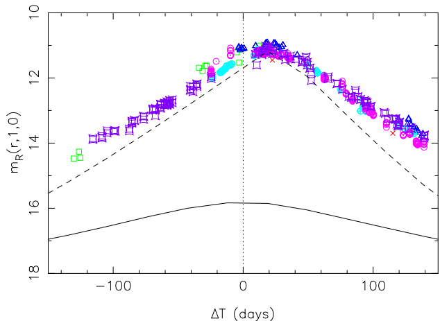
Figure 4. Same as Fig. 3, but plotted against time from perihelion (days) and showing only the near-perihelion period ( \pm 150 days).
