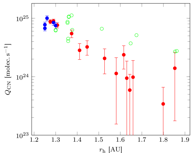
Figure 6. Post-perihelion CN production rates in comet 67P as a function of heliocentric distance with 1- \sigma uncertainties. Red symbols are measurements by LOTUS, blue from TRAPPIST, and green are points from previous orbits from Schleicher (2006).
