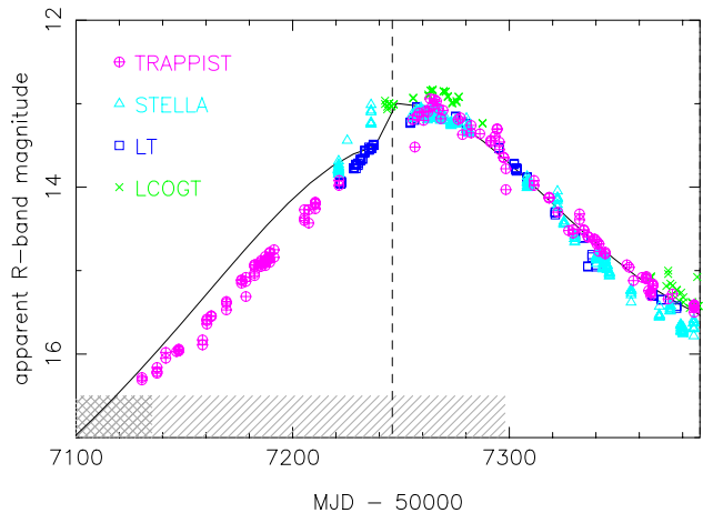
Figure 2. Same as Fig. 1, showing zoom in on 2015 period around perihelion. Here the Solar elongation is shown by shading at bottom of the plot only, for ease of seeing data points.
