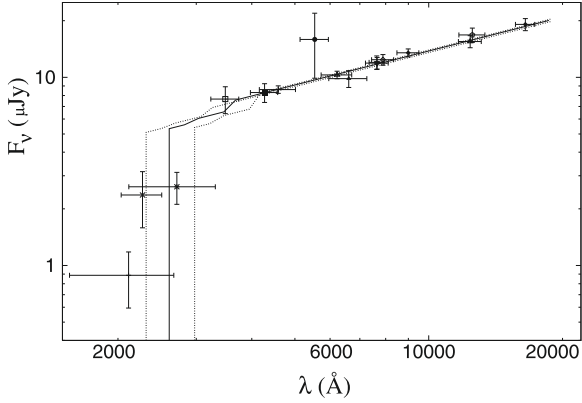
Fig. 3. The SED of the afterglow at 1 day after the burst fitted using the HyperZ tool (solid line; the dotted lines show the 1\sigma uncertainties). From left to right: UVOT uvw2 , uvm2 , uvw1 , u and b , GROND g' , UVOT v , GROND r' , R C , GROND i' , Gemini i' , I C , GROND z' , GROND J , NEWFIRM J (see Table A.1) and GROND H . The widths of the bands correspond to their approximation by a Gaussian filter (see Bolzonella et al. 2000). The UVOT v band is affected by a short exposure time, the low sensitivity of the detector at longer wavelengths and high background.
