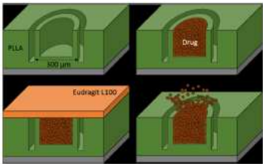
330 331 332 Fig 1 Schematic drawing of the concept of the microwells as an oral drug delivery system: a) the biodegradable 333 microwells fabricated from PLLA, b) filled with ASSF c) and subsequently spray coated with a lid of Eudragit® L100. 334 d) at pH 6.5 (intestinal pH) ASSF is released from the microwells 335
