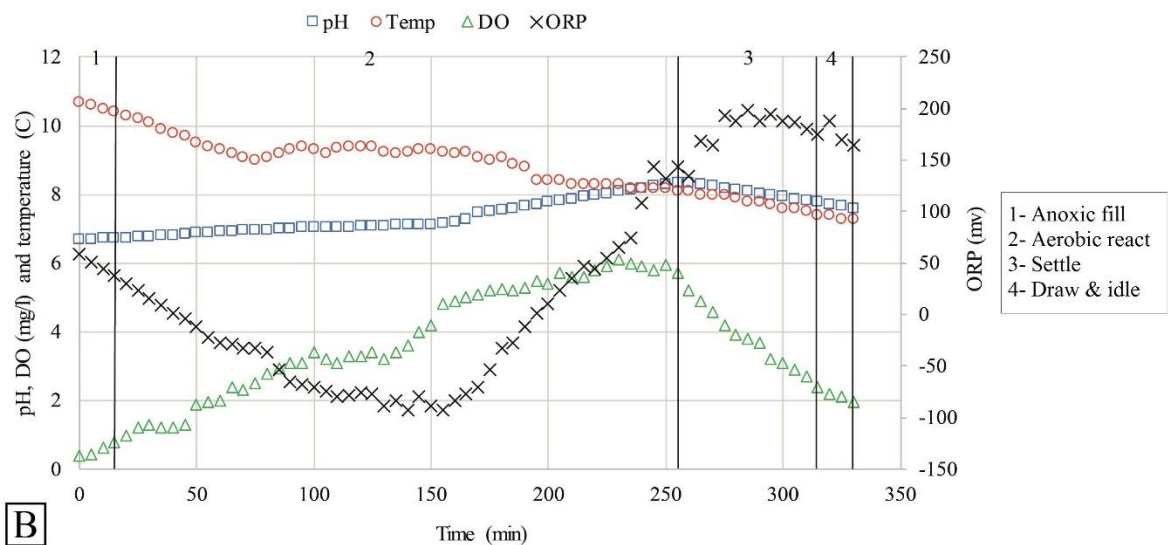
Fig. 8. pH, DO, temperature and ORP profiles for one treatment cycle of a) TSSBR, b) NOSBR.
