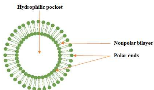
Figure 1. Liposome.
