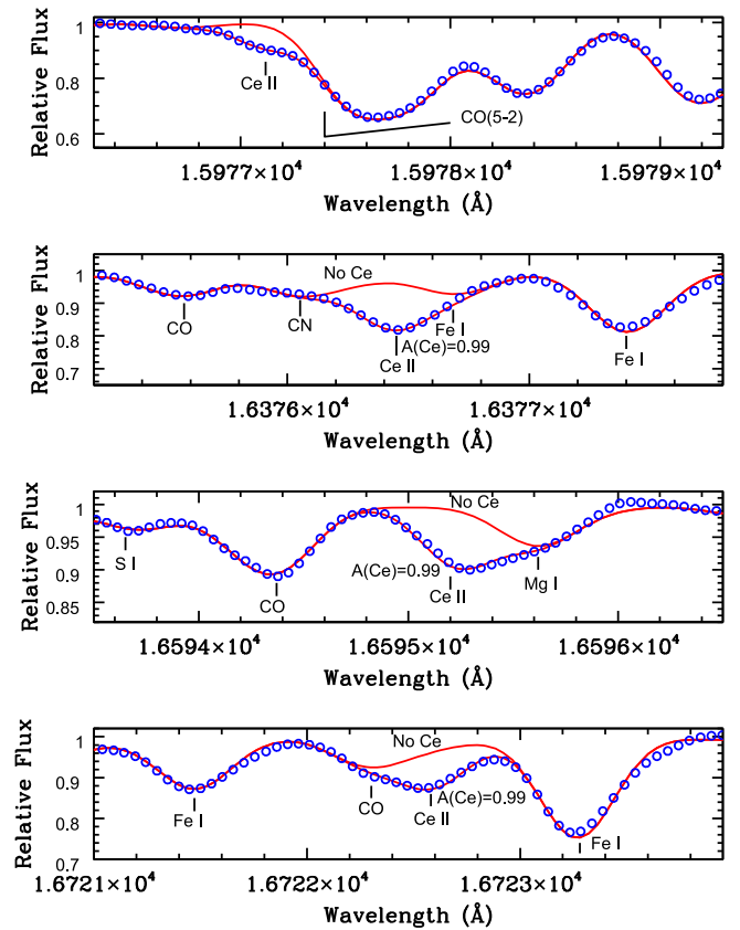
Figure 2. Four other sample Ce II lines shown in the observed FTS spectra of \alpha Boo. Same as Figure 1.
