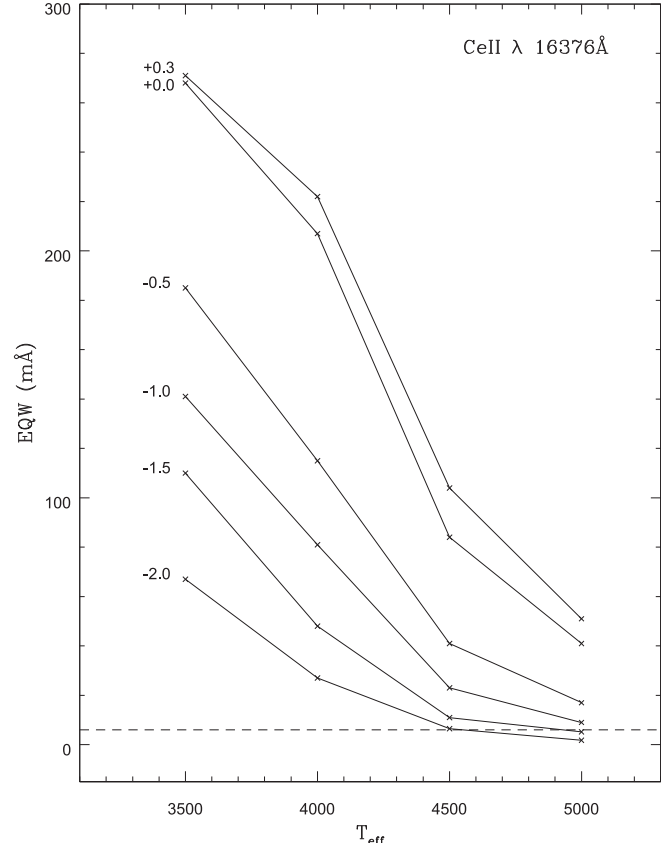
Figure 8. Equivalent width of the \lambda 16376 \text{ \AA} Ce II line as a function of T_{\text{eff}} and [\text{Fe}/\text{H}] , with each value of T_{\text{eff}} paired with a \log g value typical for a red giant ( T_{\text{eff}} = 3500 \text{ K}, \log g = 0.5 ; T_{\text{eff}} = 4000 \text{ K}, \log g = 1.0 ; T_{\text{eff}} = 4500 \text{ K}, \log g = 1.5 ; and T_{\text{eff}} = 5000 \text{ K}, \log g = 2.0 ). The Ce II equivalent widths are calculated assuming [\text{Ce}/\text{Fe}] = 0.0 . This Ce II line will be detectable in a significant fraction of APOGEE red giants. It falls below detection limits only in the hotter and quite metal-poor red giants. The horizontal dashed line indicates the approximate equivalent width detection of \sim 6 \text{ m\AA} for an APOGEE spectrum with an S/N = 100 .
