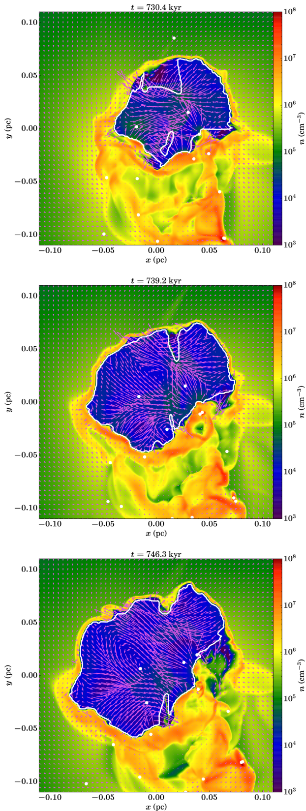
Figure 3. Snapshot density slices through the simulations of P10 after the formation of an H II region in the xy -plane. The time-steps reflect later evolutionary stages that occur at 730.4, 739.2, and 746.3 kyr. The arrows depict velocity vectors and the white points are sink particles. The thin white border marks the boundary of 90 per cent ionization fraction.
