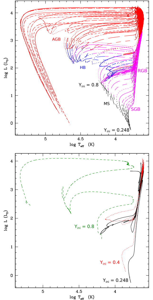
Fig. 2. Top: evolution in the HRD of the 0.8 M_{\odot} models for 16 different Y_{\text{ini}} between 0.248 and 0.8 ( Z = 5 \times 10^{-4} ). Colors depict the evolutionary phases (main sequence in black, subgiant and red giant branch in magenta, central helium burning in blue, post central helium burning in red; the pre-main sequence is not shown for clarity). Bottom: 0.8 M_{\odot} models computed with Y_{\text{ini}} = 0.248, 0.4 , and 0.8 (black, red, and green, respectively).
