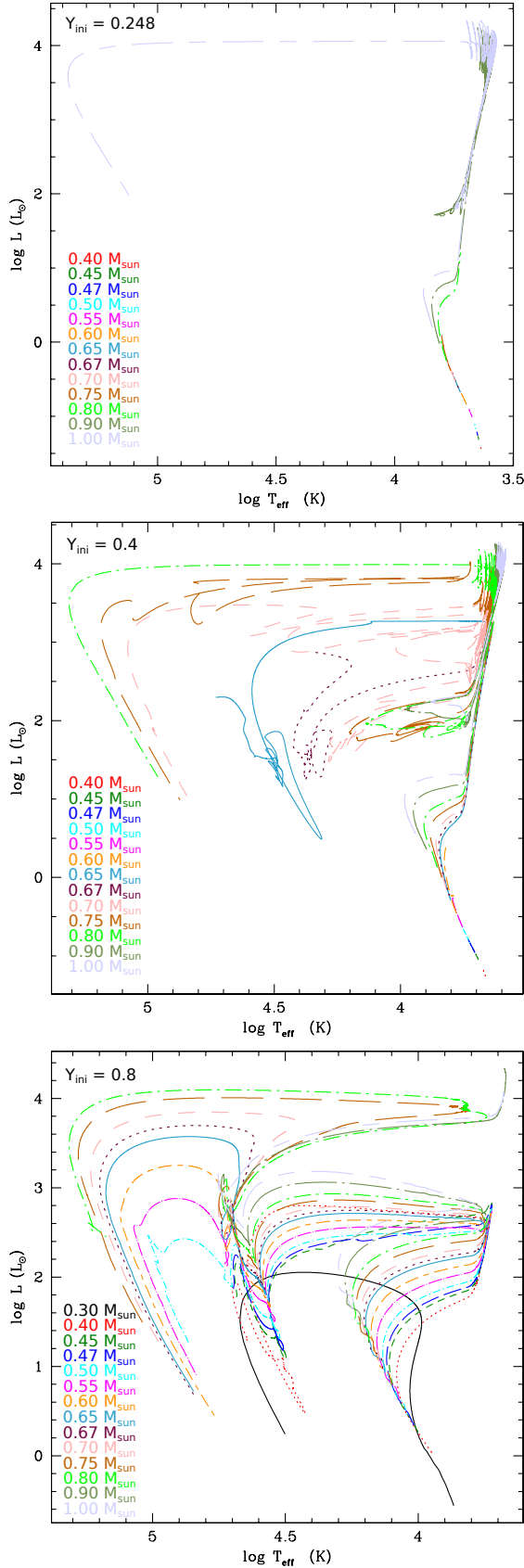
Fig. 13. Evolution in the HRD of all the models with initial stellar masses between 0.3 and 1.0 M_{\odot} for Y_{\text{ini}} = 0.248 , 0.4, and 0.8 (top, middle, and bottom, respectively). For the very low-mass models, we stop the evolution if it exceeds 14 Gyr. At this age, the (0.3, 0.248) and (0.3, 0.4) models are still on the pre-main sequence, therefore they are not present in the HRD.
