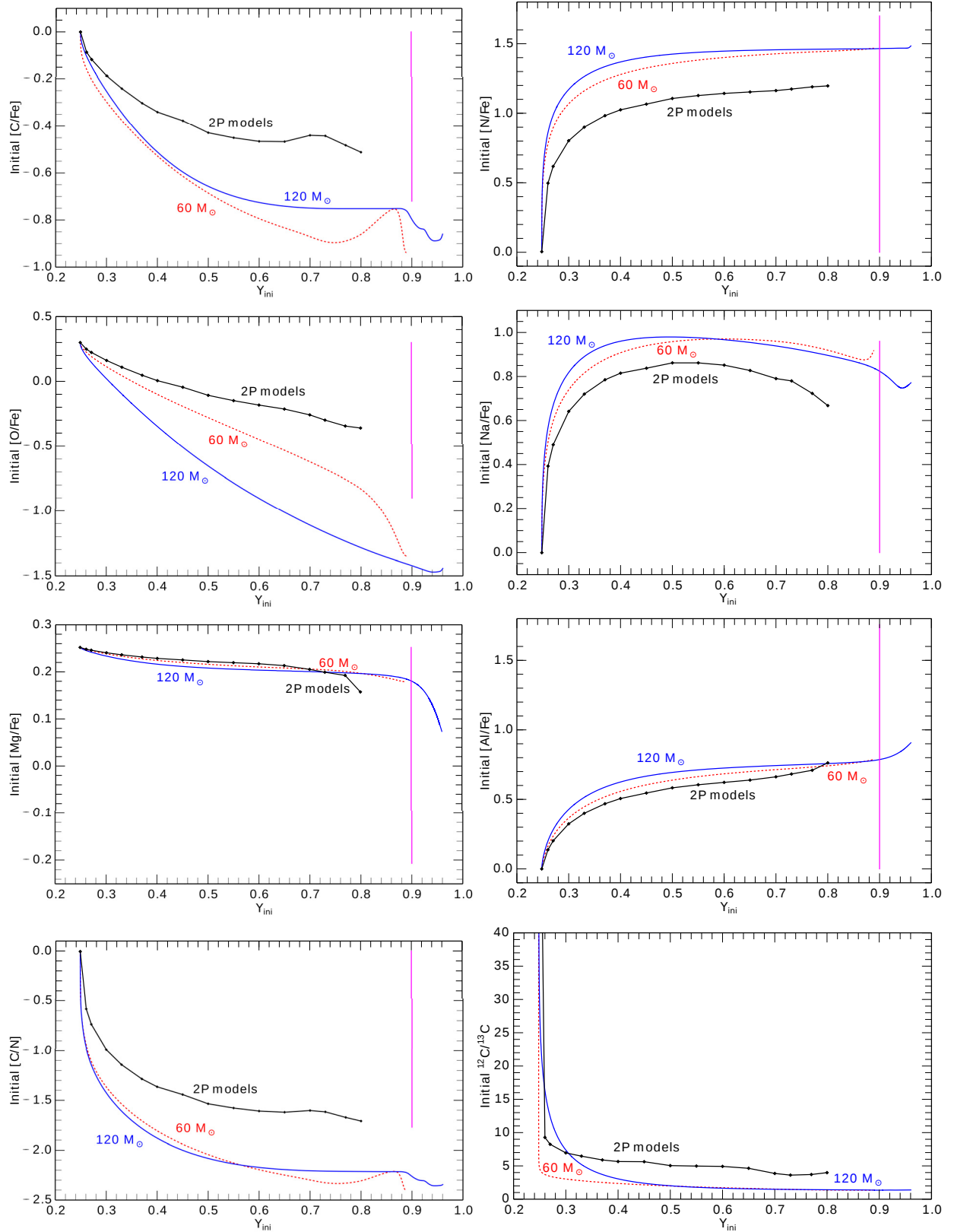
Fig. 1. Theoretical distribution for the initial carbon, nitrogen, oxygen, sodium, magnesium, and aluminum abundances ( [X/Fe] = \log(X/Fe)_* - \log(X/Fe)_\odot ) for [C/N] and for ^{12}C/^{13}C (initial value of 90) as a function of the initial helium mass fraction adopted for our 2P stars models (black line; dots indicate the 16 values adopted for the model computations of each stellar mass between 0.3 and 1 M_\odot ). This accounts for dilution between original 1P material and the ejecta of the 60 and 120 M_\odot FRMS models (red and blue lines, respectively; Decressin et al. 2007b) as described in Eq. (1) (see text). The magenta arrows represent the variations observed in NGC 6752 for [C/Fe] and [N/Fe] (Carretta et al. 2005), [O/Fe] and [Na/Fe] (Carretta et al. 2007), and [Mg/Fe] and [Al/Fe] (Carretta et al. 2012).
