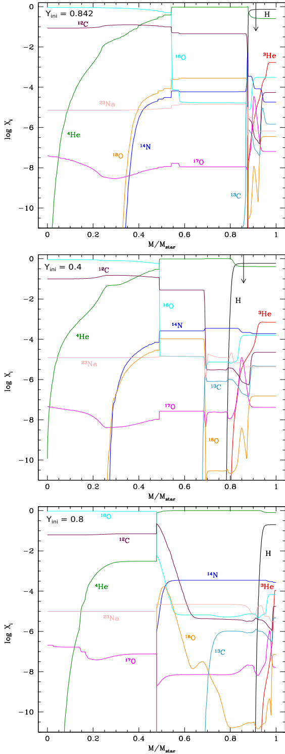
Fig. 11. Abundance profiles as a function of the depth in mass for the main chemical elements at the end of the central helium burning for the 0.8 M_{\odot} models with Y_{\text{ini}} = 0.248, 0.4 , and 0.8 (from top to bottom). The total stellar mass at this evolution point is respectively 0.573, 0.662 , and 0.772 M_{\odot} . The arrows indicate the maximum depth of the convective envelope during the early AGB phase.
