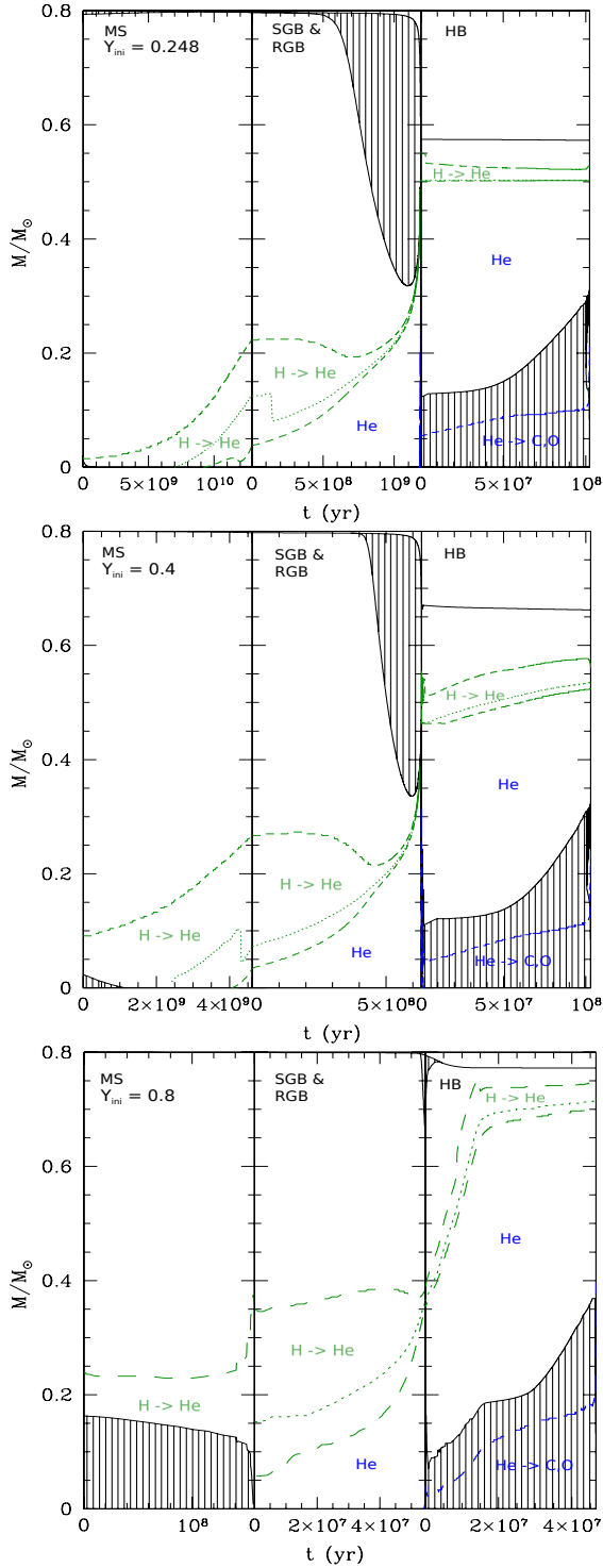
Fig. 6. Internal properties (Kippenhahn diagram) of the 0.8 M_{\odot} models with Y_{\text{ini}} = 0.248, 0.4 , and 0.8 (top, middle, bottom) from the zero age main sequence to the end of central-helium burning. Green dashed lines delimit hydrogen burning regions ( \geq 10 \text{ erg g}^{-1} \text{ s}^{-1} ); blue dashed lines delimit the helium burning regions ( \geq 10^3 \text{ erg g}^{-1} \text{ s}^{-1} ); dotted green and blue lines show the maximum energy production of H- and He-burning; hatched areas represent the convective zones. Timescales give the duration of each evolutionary phase.
