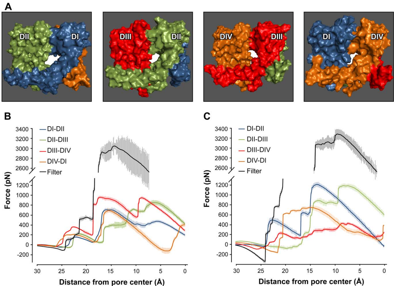
Figure 5. Side fenestrations offer a new entrance pathway. A: Surface representations of hNav1.5 side fenestrations as viewed from the membrane. The model is colored by domain with the central white region showing the fenestration located at the interface of each domain pair. B–C: Force exerted on the center-of-mass of BPA (B) or mexiletine (C) during steered molecular dynamics simulations. Each trace is the averaged force from 21 simulations displayed as mean \pm SEM. doi:10.1371/journal.pone.0041667.g005
