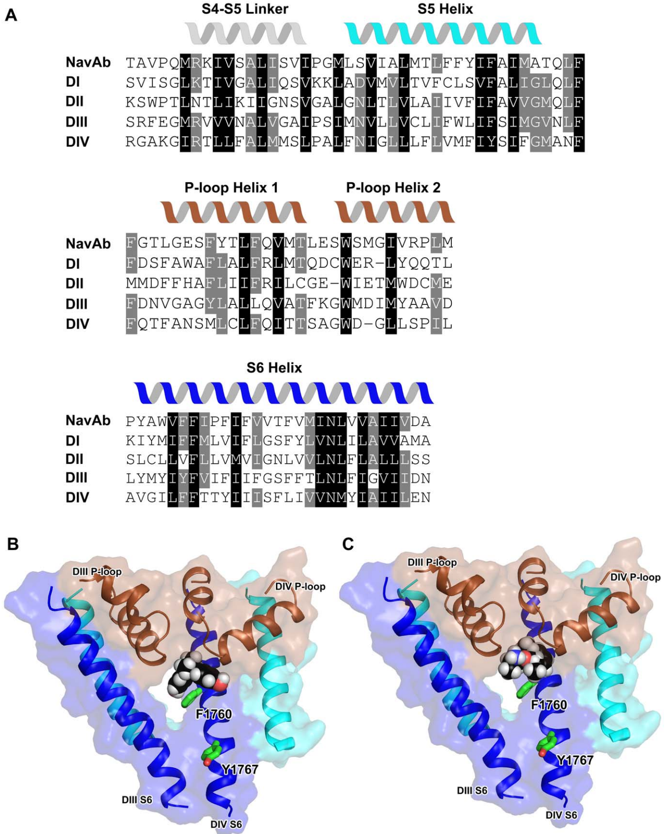
Figure 4. Modeling and ligand docking. A: Sequence alignment of the pore regions of NavAb and hNav1.5. Helical regions in the NavAb structure are indicated by the cartoons above the sequence. Residues shaded in black by sequence show high sequence homology, those in grey display moderate homology. B–C: Molecular model for the hNav1.5 structure. The protein structure is shown in ribbon mode and the ligands [(B) BPA
