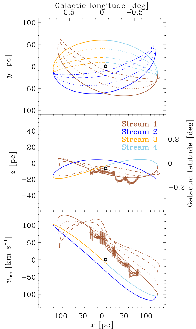
Figure 7. Comparison of the observed \text{NH}_3(1,1) emission of Stream 1 with our orbital model (lines) for different pericentre radii R_p . The \{\text{dash-dotted, dashed, dotted, solid}\} lines indicate pericentre radii of R_p = \{10, 20, 40, 59\} pc, where the latter value corresponds to our best-fitting model. As before, the colours refer to the four coherent streams in position-velocity space. The open black circle denotes the position of Sgr A*. Top row: Distribution in Galactic longitude and along the line of sight \{x, y\} . The different projected apocentre radii arise due to different heights above the plane. Middle row: Distribution in Galactic longitude and latitude \{l, b\} . Note the different scale on the y -axis compared to earlier figures. Bottom row: Distribution in Galactic longitude and line-of-sight velocity \{l, v_{\text{los}}\} . The middle and bottom panels show the effect of a changing pericentre radius only for Stream 1.
