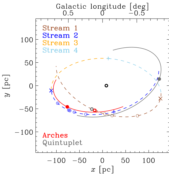
Figure 8. Top-down view of the present and past of the Arches and Quintuplet clusters in the context of our orbital model (dashed line). As in Figure 6, the observer is located in the negative- y direction. The colours again refer to the four coherent streams in position-velocity space, the thin circles indicate the implied positions in the Galactic plane of several GMCs and cloud complexes in the CMZ, the plus symbols indicate pericentres, the crosses mark apocentres, and the open black circle denotes the position of Sgr A*. The present-day positions of the Arches and Quintuplet clusters are represented by the thick circles on Stream 1, close to pericentre. The formation sites of these clusters as implied by their ages are indicated by the solid dots on lines running in parallel to the orbital model. The lengths of the lines indicate the uncertainty ranges implied by the age measurements.
