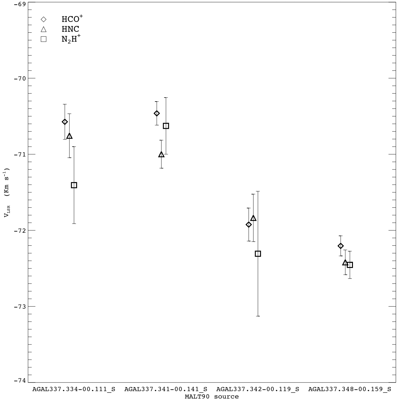
Figure 2. The central velocity from Gaussian fits of the 1-0 transitions of HCO + , HNC, and N 2 H + toward the central positions of the four ATLASGAL clumps associated with G337.342-0.119.
