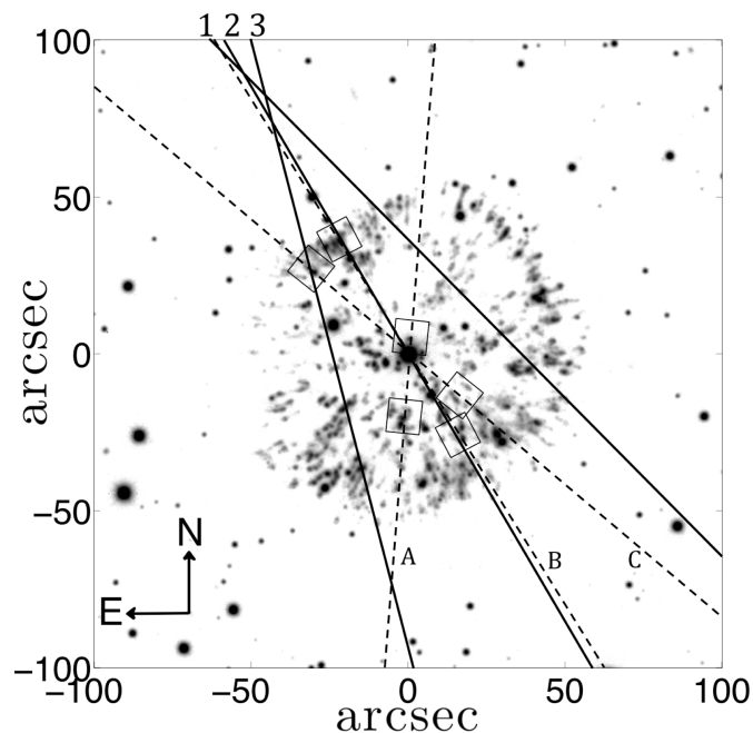
Fig. 1. Positions of the slits from MES-SPM overlaid on the stacked H\alpha Mayall image first presented in Shara et al. (2012). The slit marked 1 was placed at a PA of 45^\circ , slit 2 at 30^\circ and slit 3 at 9^\circ . All three slit positions cover the jet-like feature to the NE of the nova remnant as well as sections of the nova shell. Slit 1 & 2 observations were obtained on 2014-Nov-28 and slit 3 on 2015-Mar-27/28, see Table 2a. Slits marked A, B, and C are those at PA = 173^\circ , 31^\circ , and 49^\circ , respectively. It is from these slit positions that the P-V arrays were simulated in Figs. 2–4. The overlaid boxes cover the knots used in the same figures.
