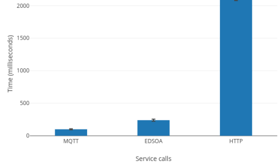
Fig. 4. The average end-to-end delay with a single sensor device. Vertical bar signifies the SVL/PAL and the event manager in 3SOA and EDSOA respectively.
