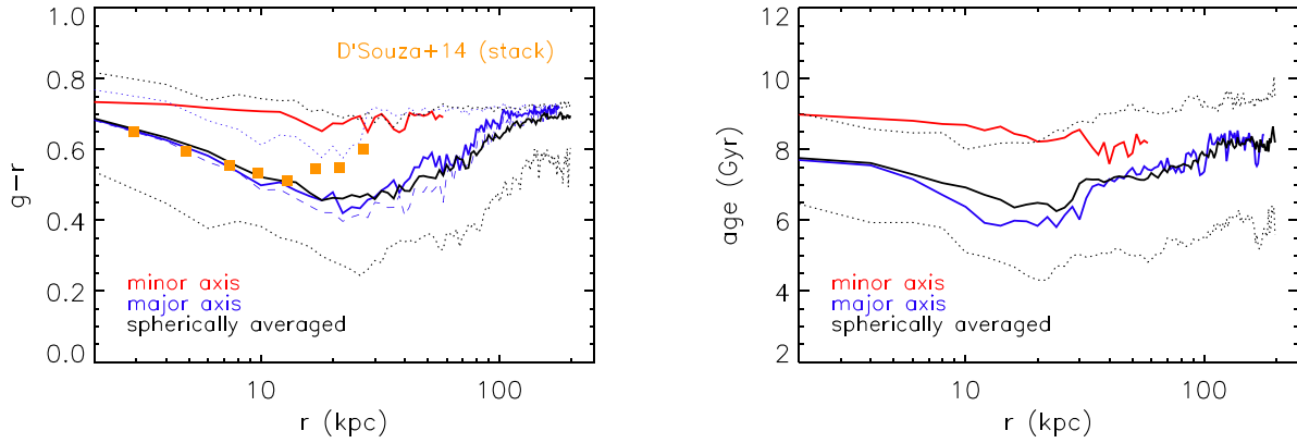
Figure 7. Left: A comparison between simulated g-r profiles and observations. The solid coloured curves represent the median colour along the major axis (blue), along the minor axes (red), and spherically averaged (black). The dotted blue and dashed blue curves represent the median major axis profiles for the accreted and in situ components, respectively. The black dotted curves show the corresponding galaxy-to-galaxy scatter (16th and 84th percentiles) for the spherically averaged case. The filled orange squares show the azimuthally averaged g-r colour of Milky Way-mass galaxies in SDSS DR9 from D’Souza et al. (2014). Right: The median age profile of the simulated galaxies. The coloured curves have the same meaning as in the left-hand panel.
