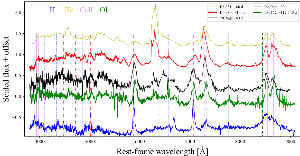
Figure 13. The +140.7 d spectrum of SN 2018gix compared with SNe I1b 2015G (Shivvers et al. 2017b) and 2006jc (Pastorello et al. 2008b) and Type I1b SN 1993J (Matheson et al. 2000a) and SN 2008bo (Modjaz et al. 2014). The spectra of SN 2008gix, SN 2006jc, and SN 2015G are binned to \sim 3 Å for clarity. The key difference between the nebular spectra of SNe I1b and those of the interaction dominated SNe I1b can be seen in the strength of the [O I] \lambda\lambda 6300, 6364 feature, as well as the strength of the He I lines.
