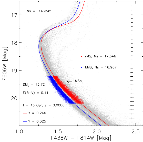
Fig. 1. F606W , F438W-F814W CMD from the photometric catalog of Bellini et al. (2017b). The selected samples of blue and red MS stars are marked with blue and red dots, respectively. Two isochrones from the BASTI database with different helium content and the same metallicity and age are overplotted.
