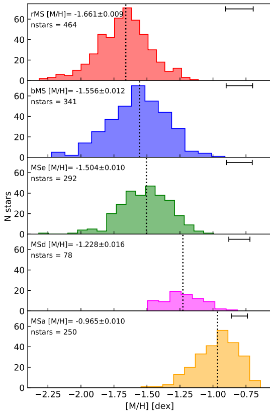
Fig. 3. Normalized metallicity distributions for the stars with S/N > 20 belonging to the five MSs defined by BE17. The mean [M/H] value (dotted line) of the distributions and the number of stars included are indicated in each panel. The horizontal bars in the top right corner show the median value of the corrected [M/H] uncertainties.
