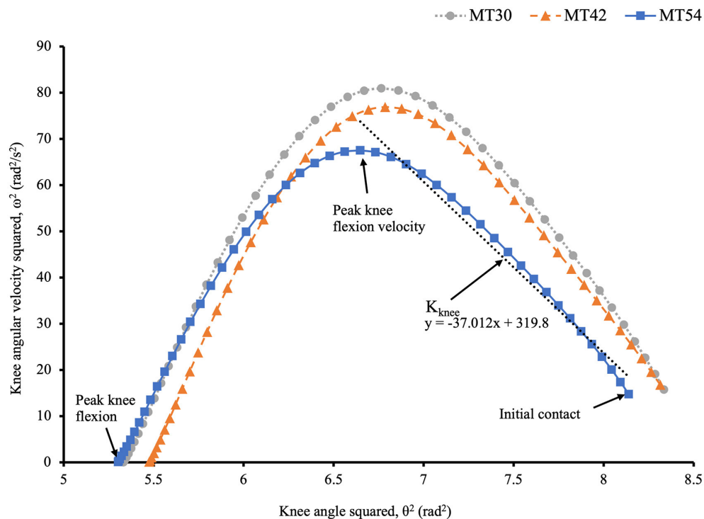
FIGURE 2 | The relationship between \omega^2 and \theta^2 of knee joint on a typical subject trial between shoe conditions during the first half of stance. Notice the two distinct sub-phases with the upward part of the curve from IC representing the impact phase and the downward part represents a weight acceptance phase (not covered in this paper). \Delta(\omega^2) / \Delta(\theta^2) for knee joint stiffness calculation was determined as the slope of the regression line shown above (i.e., the coefficient of the regression equation) throughout 20–80% of the data points (the most linear portion) of the impact phase.
