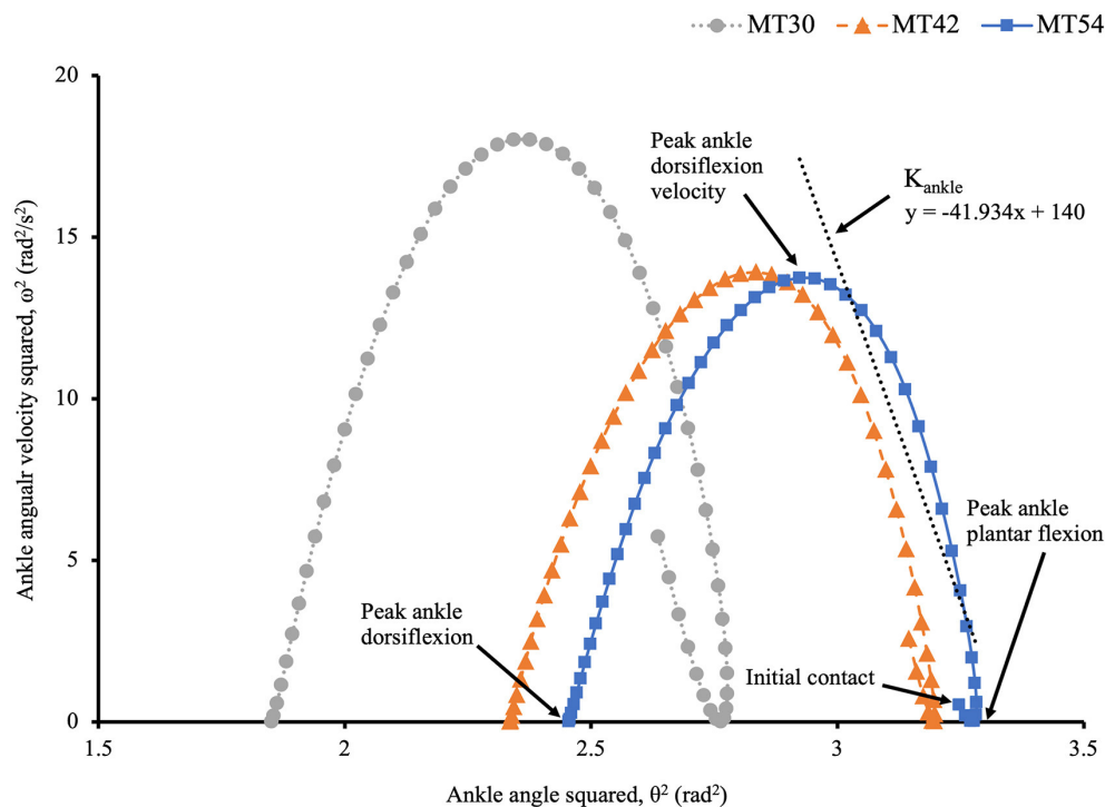
FIGURE 3 | The relationship between \omega^2 and \theta^2 of ankle joint on a typical subject trial between shoe conditions during the first half of stance. \Delta(\omega^2)/\Delta(\theta^2) for ankle joint stiffness calculation was determined as the slope of the regression line shown above (i.e., the coefficient of the regression equation) throughout 20–80% of the data points (the most linear portion) of the impact phase.
