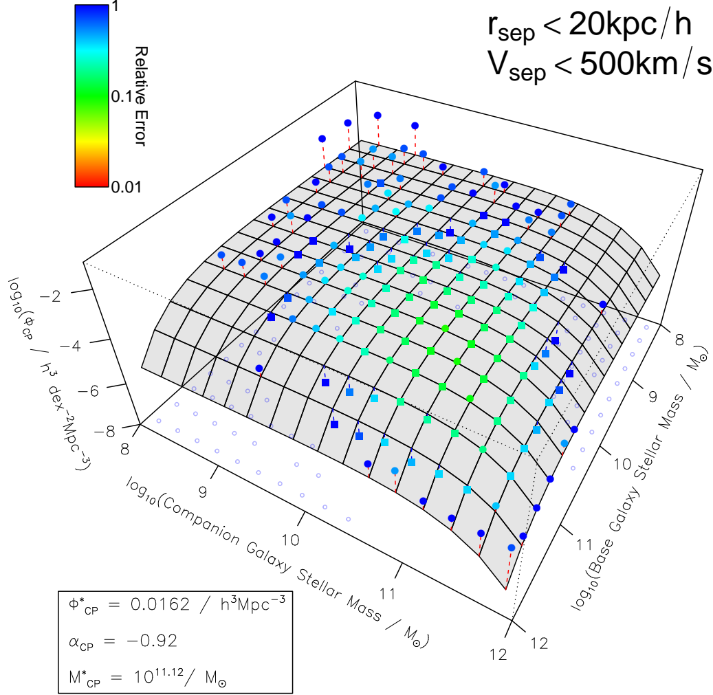
Figure 10. Fit to the 2D close-pair density distribution for r_{\text{sep}} < 20 \text{ kpc} and v_{\text{sep}} < 500 \text{ km s}^{-1} sample ( PS_{r20v500} ) as observed, i.e. not true pair corrected using the mock catalogues (see Section 3.4). The fit is represented by the grey shaded 2D manifold. The colour of the binned data represents the estimated relative error (so redder points dominate the fit more). Circles on the base of the 3D plot represent missing data.
