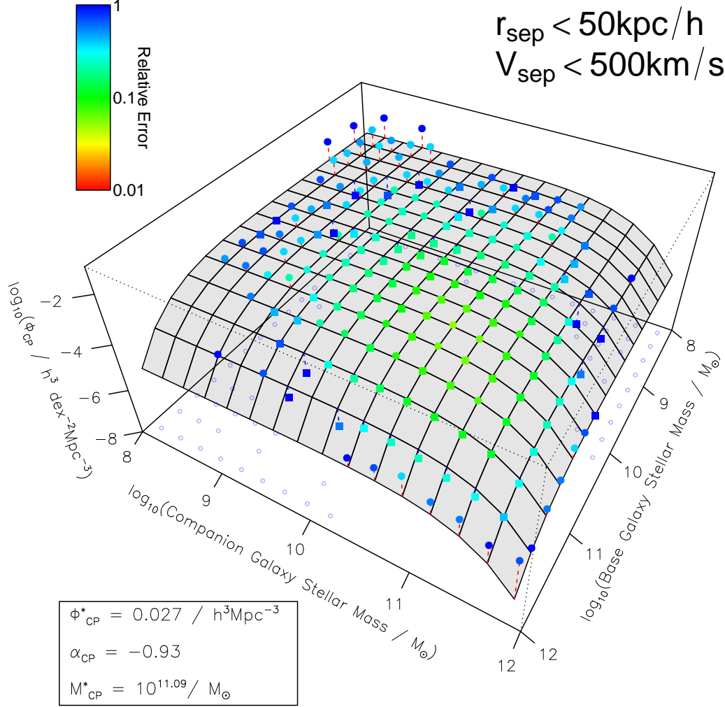
Figure 11. Fit to the 2D close-pair density distribution for r_{\text{sep}} < 50 \text{ kpc} and v_{\text{sep}} < 500 \text{ km s}^{-1} sample ( PS_{r50v500} ) as observed, i.e. not true pair corrected using the mock catalogues (see Section 3.4). See Figure 10 for details.
