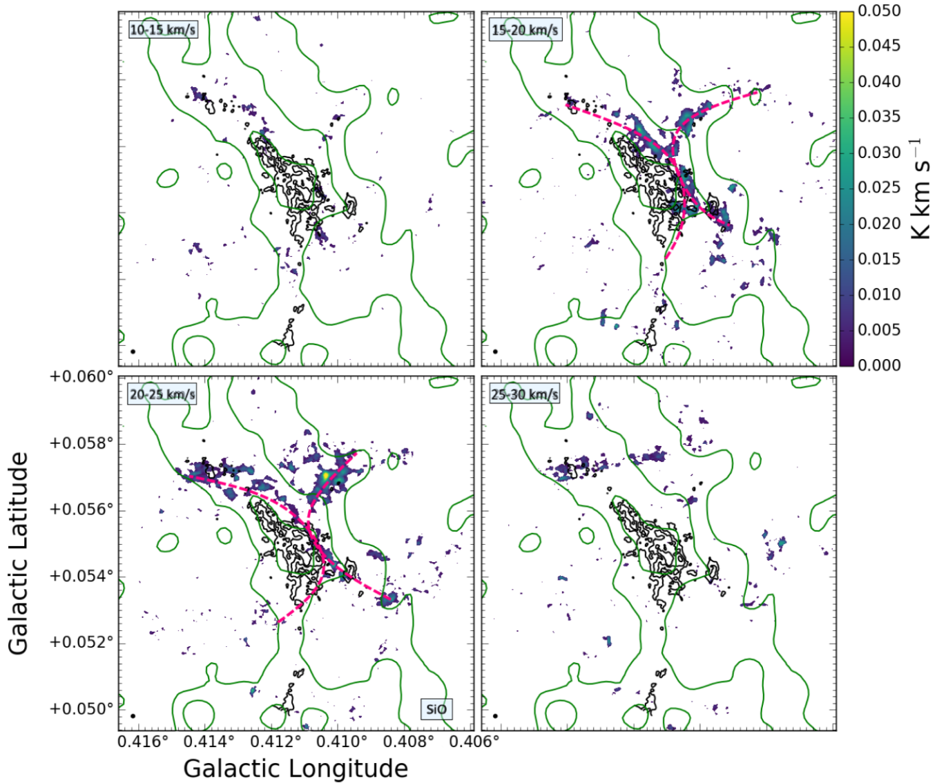
Figure 12. A channel map of SiO from our ALMA data in the range of 10–30 km −1 . Black contours show the dust continuum of our ALMA data and green contours show SMA 1.3 mm continuum data. The black circle in each plot represents the synthesized beam. Magenta dashed lines show the ‘hollow circle’ features described in Section 4.3. The velocity gradient seen on larger scales in cloud ‘d’ can be seen on this smaller scale.
