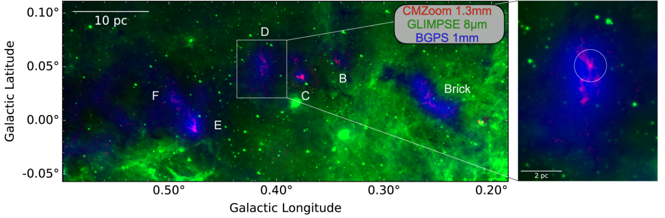
Figure 1. Left: Three-colour image of the Galactic Centre dust ridge. Red: SMA 1.3 mm dust continuum (Battersby et al. 2020), Green: Spitzer/GLIMPSE 8 \mu\text{m} emission (Churchwell et al. 2009), Blue: Bolocam Galactic Plane Survey 1 mm dust continuum (BGPS, Ginsburg et al. 2013). Right: Zoom-in on dust ridge cloud ‘d’ (G0.412 + 0.052). The white circle corresponds to the primary beam field of view of the ALMA observation towards source ‘d6’ (Walker et al. 2018) reported in this paper.
