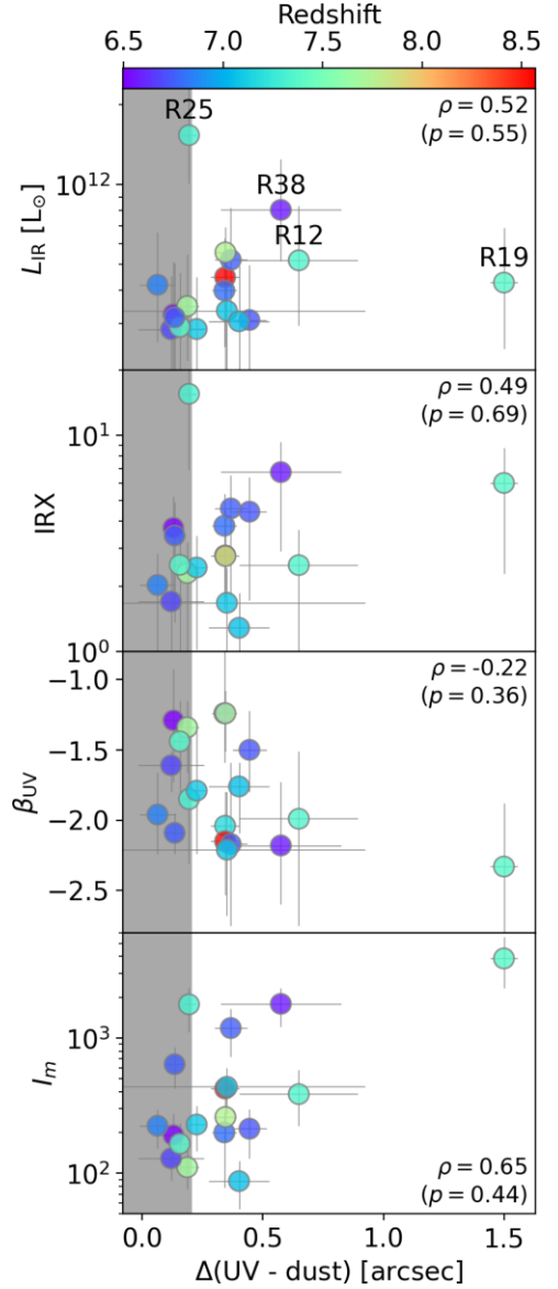
Figure 8. Galaxy physical properties against spatial offsets. From the top to bottom, IR luminosity ( L_{IR} ), UV spectral slope ( \beta_{UV} ), infrared excess ( IRX ), and molecular index ( I_m ). The symbols are colour coded by their spectroscopic redshifts where available, and the others are photometric redshifts. The grey region indicates the separation below the expected astrometric uncertainty of the ALMA observations (see Section 2.1). The Spearman rank correlation coefficient ( \rho ) and the associated p -value are shown in each panel.
