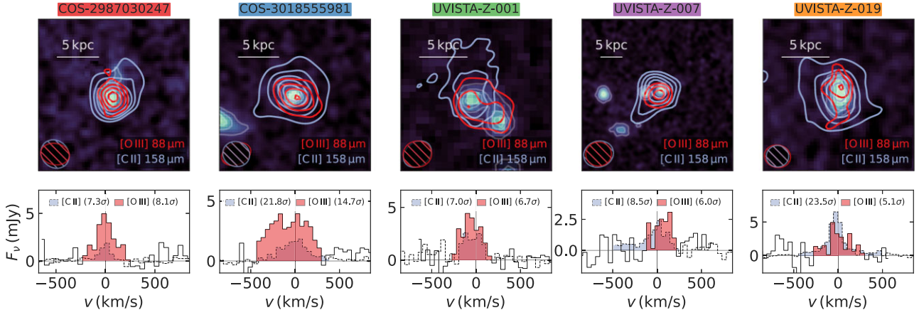
Figure 2. Detections of the [C II] 158- and [O III] 88- \mu\text{m} lines. Top row: contour images of the [C II] and [O III] lines overlaid on a background of HST rest-frame UV images (see Section 2.3). The line images have matched beam sizes (as listed in Table 2) and are produced by collapsing all channels within the FWHM of the line (as those of the S/N determination, which however use natural weighting without tapering; Section 3.3). Contours start at 3\sigma and increase in steps of 5\sigma for the [C II] contours in COS-3018555981 and UVISTA-Z-019, 3\sigma for the [O III] contours in COS-3018555981, 2\sigma for both lines in UVISTA-Z-001, and 1\sigma otherwise. Bottom row: S/N-weighted line spectra extracted from a 2\sigma region in a naturally weighted image integrated over the FWHM (cf. Section 3.3). Coloured channels, which were used to produce a subsequent moment-zero map for measuring the total line flux, indicate the line detection. The significance of each line detection is shown in the legend (also see Section 3.3 for details).
