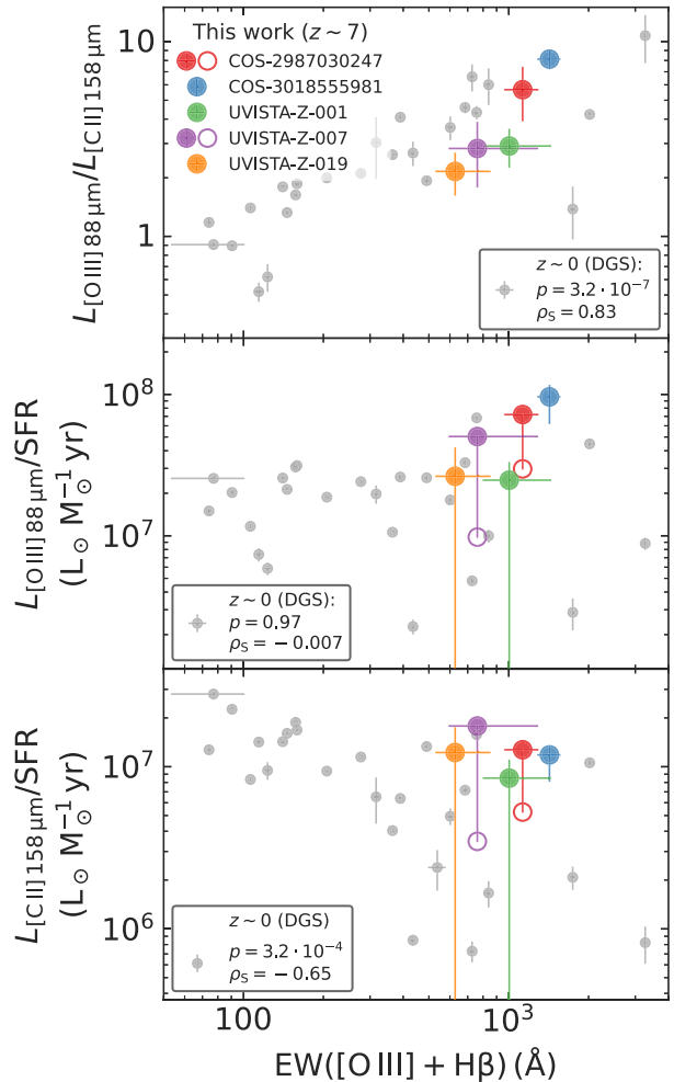
Figure 6. Ratios of the [O III] 88- and [C II] 158- \mu\text{m} luminosities with respect to each other (top panel) and with respect to the SFR (middle panel for [O III], bottom panel for [C II]) as a function of the EW of the optical [O III] and H\beta lines. If the measured SFR is an upper limit (due to a non-detection of the dust continuum), unobscured SFR measurements are shown with an open circle. Small grey circles are galaxies from DGS (see Section 5.2). The p -value, for a null hypothesis that the data are uncorrelated, and Spearman’s rank correlation coefficient ( \rho_s ) of these points measured in logarithmic space are indicated in each panel. Coloured circles show the five z \sim 7 galaxies considered in this work. There is a significant positive correlation between the [O III]/[C II] ratio and their optical EW among the DGS galaxies, which seems to derive mostly from a negative correlation between [C II]/SFR and the EW; however, the correlation of the [O III]/[C II] luminosity ratio is stronger than that of the (relative) [C II] luminosity on its own. Furthermore, it is unclear whether the same is true for the small sample of high-redshift galaxies.
