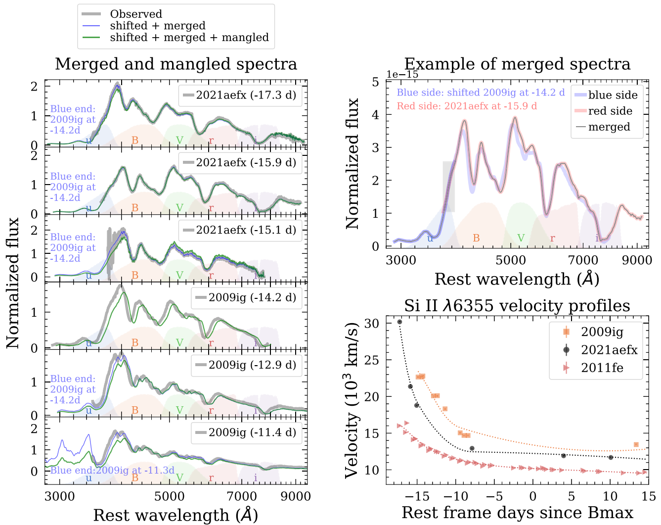
Figure 3. (Left): the six color-adjusted spectra chosen for this analysis, including three early spectra of SN 2021aefx and three spectra of SN 2009ig. The spectra are color matched to the observed photometry of SN 2021aefx. (Top right): an example of the merging process between SN 2021aefx and SN 2009ig. Before the merging process, the spectra of SN 2009ig are shifted in velocity to match the velocity of SN 2021aefx at the same phase. The gray shade marks the overlapping region used to match the flux scale. (Bottom right): Velocity profiles of the minimum of the Si II \lambda 6355 feature in SN 2011fe, SN 2009ig, and SN 2021aefx.
