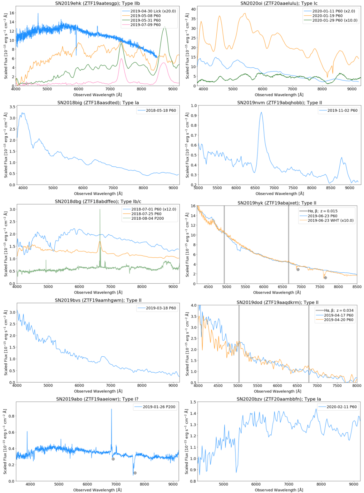
Figure 3. Selected epochs of P60 +SEDM (or P200 ) spectroscopy that are relevant to the classification of SN siblings with peak observed magnitude \leq 18.5 mag in either the g or r filter (the gold sample). For SN 2019ehk we also include the classification spectrum from Lick Observatory (Dimitriadis et al. 2019). For SN 2018dbg, the 2018-08-04 spectrum was published in De et al. (2021). For SN 2019hyk, we also include the classification spectrum from the William Herschel Telescope (WHT; Fraser et al. 2019).
