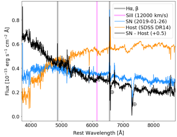
Figure 4. The spectrum of AT 2019abo from Fig. 3 (blue), the host galaxy spectrum from SDSS DR14 (Abolfathi et al. 2018; orange), and the host-subtracted SN spectrum (host galaxy) (black). Grey and magenta lines mark the locations of hydrogen emission (host galaxy) and potential Si II \lambda 6355\text{\AA} absorption (a signature SN Ia feature), respectively. Earth symbols mark two strong atmospheric absorption features.
