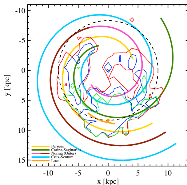
Figure 3. The same as Fig. 2, but with source density contours displayed instead of source positions. Sources are counted in boxes of 1 \text{kpc}^2 . To avoid figure crowding, only one contour, corresponding to a level of 100 sources \text{kpc}^{-2} is plotted for each source class: green for starless unbound sources (not shown in Fig. 2), red for pre-stellar, and blue for protostellar, respectively.
