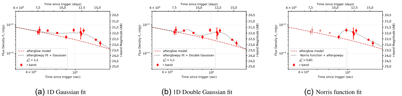
Figure 9. Late-time excessive emission fitting with various models. (a) A simple Gaussian fitting to the peak. (b) A double Gaussian fit to the late-time variability. (c) Norris function fitted on the two peaks for flaring. The solid dark markers shows the data used for fitting for a particular function.
