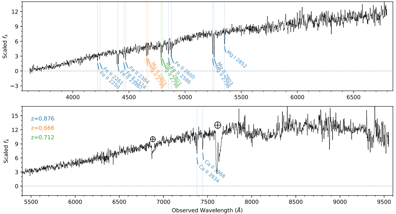
Figure 3. GMOS-S spectrum of ZTF21 aagwbjr. The upper and bottom panels show the resulting spectrum in the blue and red gratings, respectively. We identify a number of strong, narrow absorption features of Fe II, Mg II, M I, and Ca II at a common redshift of z = 0.876 (blue notations). We identify two additional intervening absorbers, based on Mg II \lambda\lambda 2796, 2803 at z = 0.666 (orange notations) and z = 0.712 (green notations).
