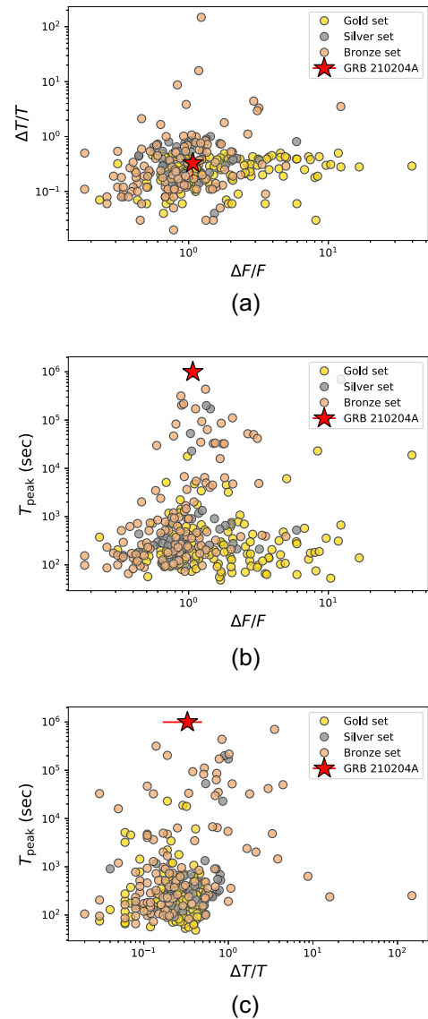
Figure 11. Comparison of flaring properties of GRB210204A with GRB flares published in Swenson & Roming (2014). The gold, silver, and bronze sets are shown by respective colors. GRB 210204A is depicted with a red star symbol, with the limits of the error bar, indicating the two \Delta t values measured in Section 4.3. The flare is very similar to other flares in terms of \Delta F/F and \Delta t/t , but occurs later than any of the flares in the Swenson & Roming (2014) data set.
