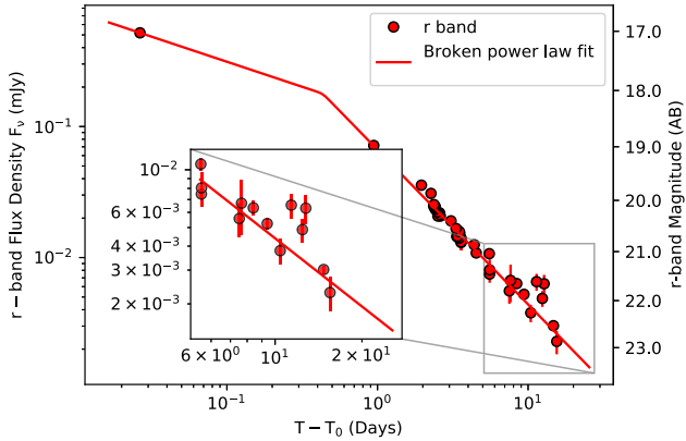
Figure 6. Broken power-law fit on r-band afterglow light curve. The red dots depicts the data points in r-band and the solid line is a broken power-law fit on the data. The inset shows a zoomed-in version of the light curve where it shows significant deviation from power-law around T - T_0 \sim 10 d.
