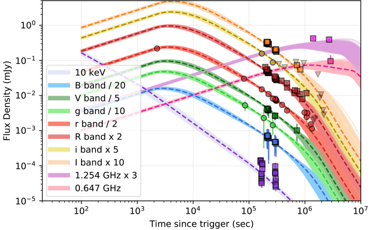
Figure 7. A multiband light curve of GRB 210204A afterglow. The multiband light curve of the GRB 210204A afterglow was fitted to the data using the AFTERGLOWPY package integrated with the AFTERGLOWPY with EMCEE PYTHON package for MCMC. Dotted lines show the best-fitting light curve to each band, and the light coloured band around the dotted line indicates the 16 per cent and 84 per cent quantiles uncertainty in the fitting.
