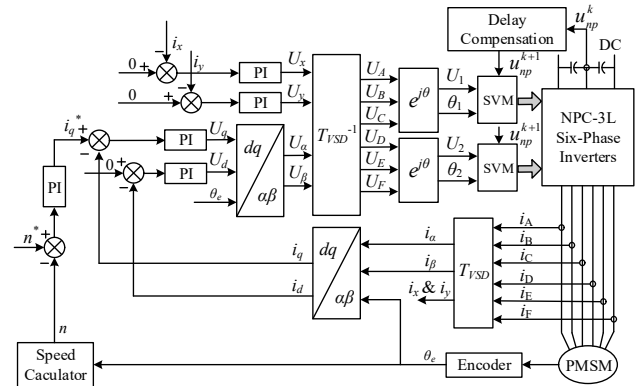
Fig. 2. Diagram of the basic control scheme.
