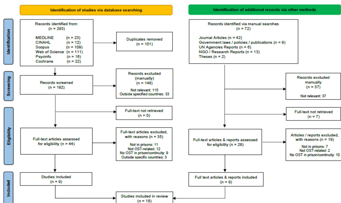
Fig. 1. PRISMA flowchart.
